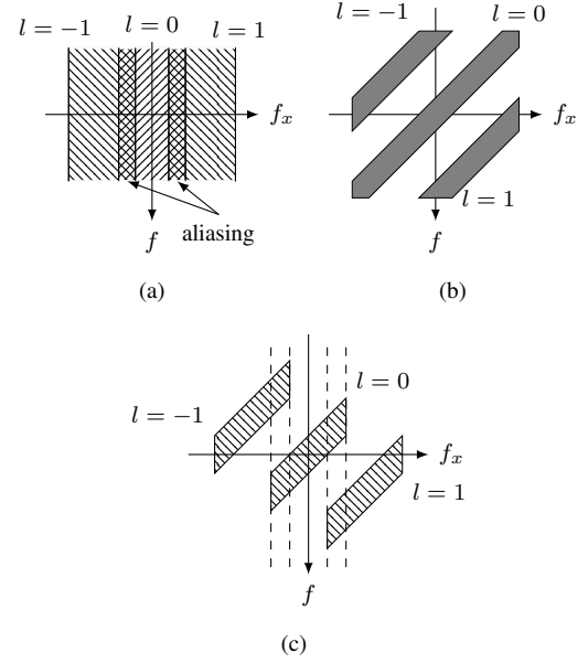
Fig. 1. The support of the spectrum. The Fig. (a) is the sampled filtered signal spectrum support. This spectrum is defined only on f_x and is extended along the f axis. The Fig. (b) is the support of the central lobe of the sinc functions. The data spectrum is illustrated on Fig. (c). It is the sum of the product of each l -replication of the signal with the corresponding l -replication of the sinc function described by (11).
