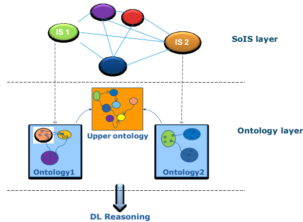
Fig. 1. Proposed approach
