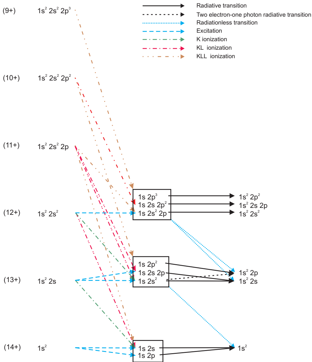
FIG. 2: Excitation, ionization and decay processes considered in this work: K excitation (- - -); single K ionization (- · · -); double KL ionization (- · · · -); triple KLL ionization(- · · · · -); radiative decay (—), and radiationless decay(· · ·).
