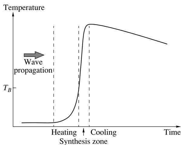
Fig. 13. Typical temperature profile of SHS process. It is the mean temperature variation for each particle in the reacting sample.
