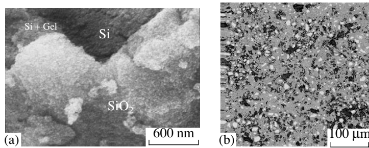
Fig. 17. SEM micrographs of (a) a raw mixture for \text{Si}_2\text{N}_2\text{O} synthesis and (b) p-SiAlON obtained by SHS under 6 MPa of nitrogen.
