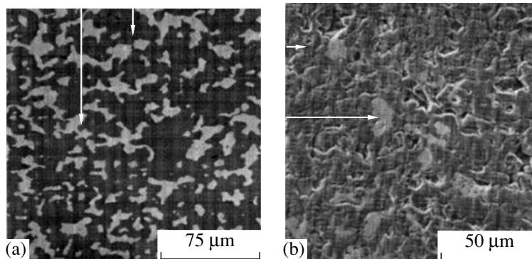
Fig. 18. Microstructure of two dense Al 2 O 3 -MoSi 2 composites: (a) 66.7% Al 2 O 3 /33.3% MoSi 2 (molar) and (b) 54.5% Al 2 O 3 /45.5% MoSi 2 (molar).
