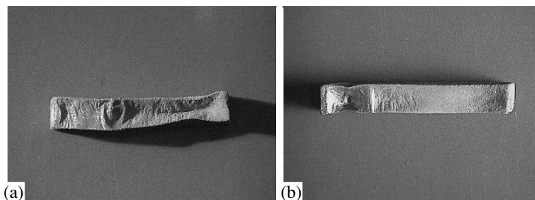
Fig. 10. TiN samples SHS-produced at two compaction pressures of green bodies: P_{\text{comp}} = 50 (a) and 150 (b) MPa [41].
