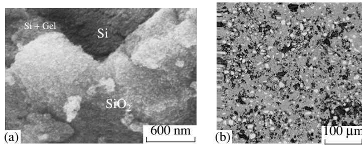
Fig. 17. SEM micrographs of (a) a raw mixture for Si 2 N 2 O synthesis and (b) p-SiAlON obtained by SHS under 6 MPa of nitrogen.
