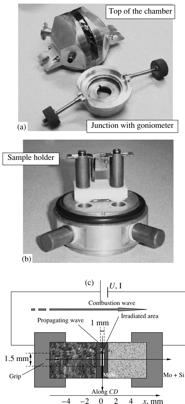
Fig. 2. (a) Reaction chamber, (b) sample holder affording to pass an electric current through the sample, and (c) schematic of SHS experiment, including sample position and positions of IR thermograms recorded during the process along AB ( x_1 , x_2 , x_3 ) and along CD [3].
