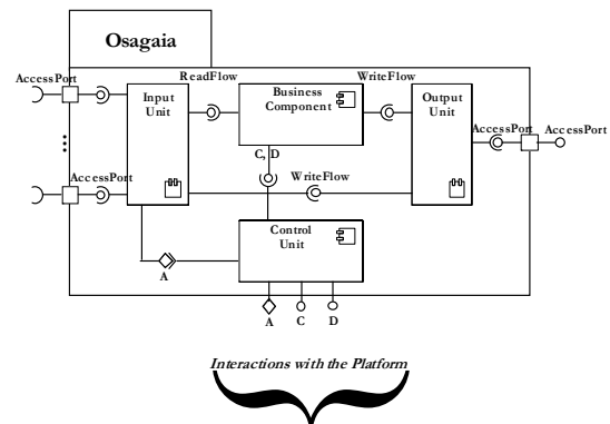
Figure 21: Osagaia Conceptual Model
