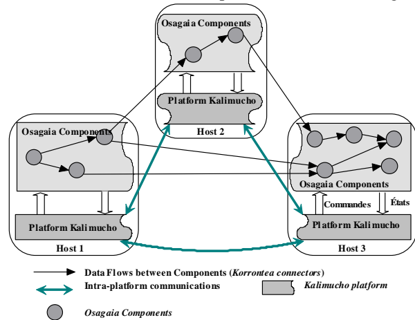
Figure 19: Kalimucho's General Architecture
