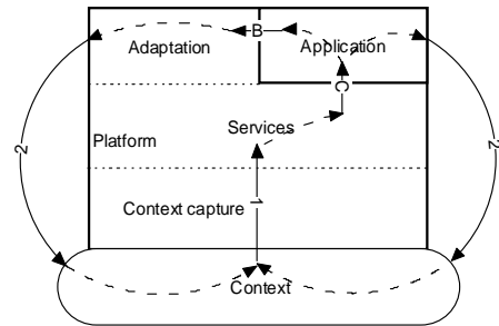
Figure 16: Non intrusive adaptation model
