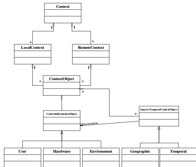
Figure 4 : Context class diagram
