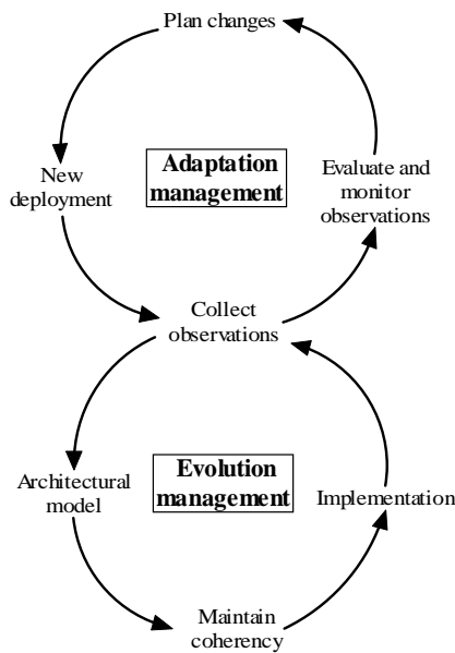
Figure 18 : General schema of adaptation [3]
