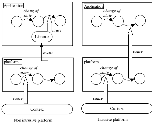
Figure 12 : Modes of interaction between platform and application
