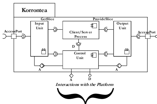
Figure 22: Korrontea Conceptual Model
