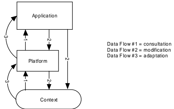
Figure 9 : Adaptable Context Aware Application with platform
