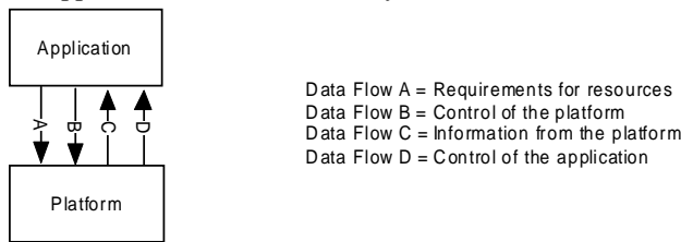
Figure 13: Information flows between application and platform [1]
