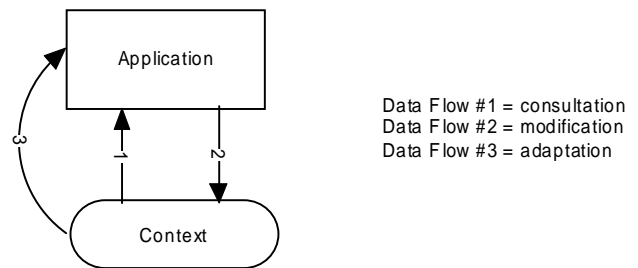
Figure 7 : Adaptable Context Aware Application
