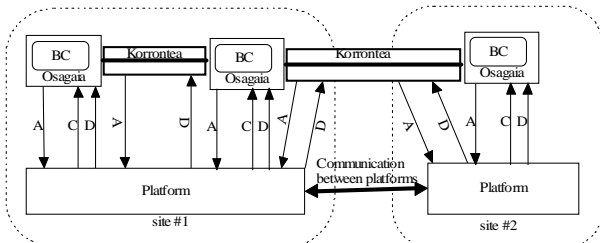
Figure 20 : Interactions between application and platform in Kalimucho
