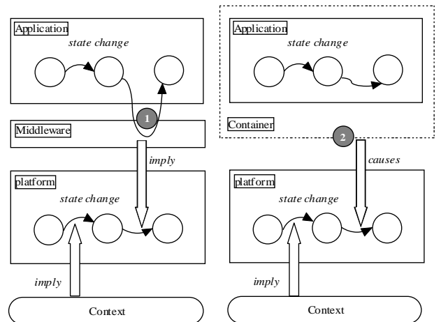
Interaction platform/Application by services Interaction platform/Application by container
