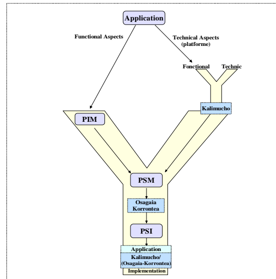
Figure 23: Model Driven Approach
