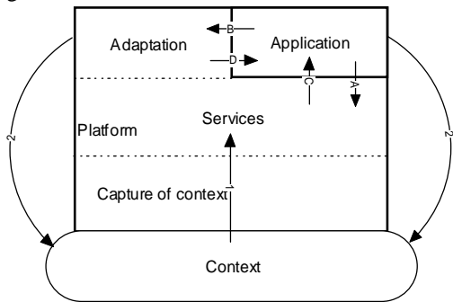
Figure 15: General schema of adaptation with a platform
