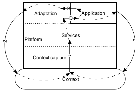
Figure 17: Intrusive adaptation model
