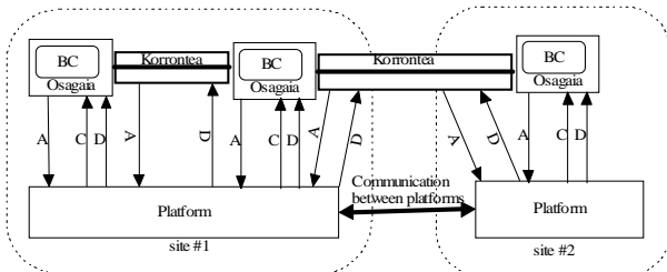
Figure 20 : Interactions between application and platform in Kalimucho
