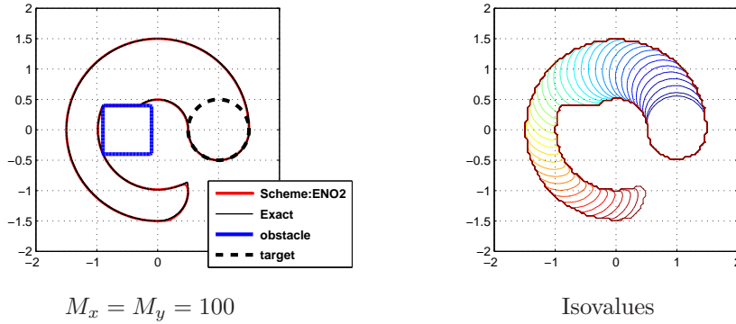
FIG. 6.2. (Example 1) Backward reachable set, t = 0.75 , with second-order ENO2 scheme (left), and isovalues (right).
