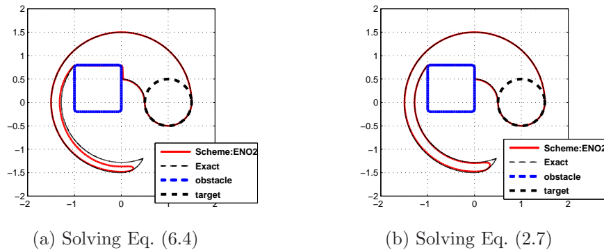
FIG. 6.3. (Example 1) Backward reachable set, t = 0.75 , with second order ENO2 scheme, (a) solving Eq. (6.4) and (b) solving Eq. (2.7), M_x = M_y = 100 .
