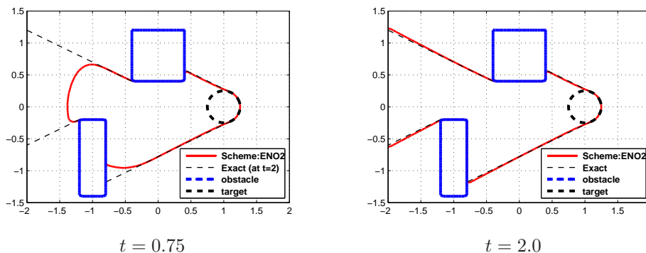
FIG. 6.4. (Example 2) Reachable set for the Zermelo problem with obstacle, at t = 0.75 (left) and at t = 2.0 (right). The computational domain is [-2, 2]^2 , and M_x = M_y = 100 .
