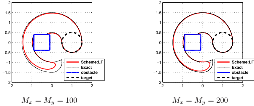
FIG. 6.1. (Example 1) Backward reachable set, t = 0.75 , with first-order LF scheme.
