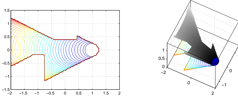
FIG. 6.5. (Example 2) Isovalues of the minimal time function, and corresponding 3d view.
