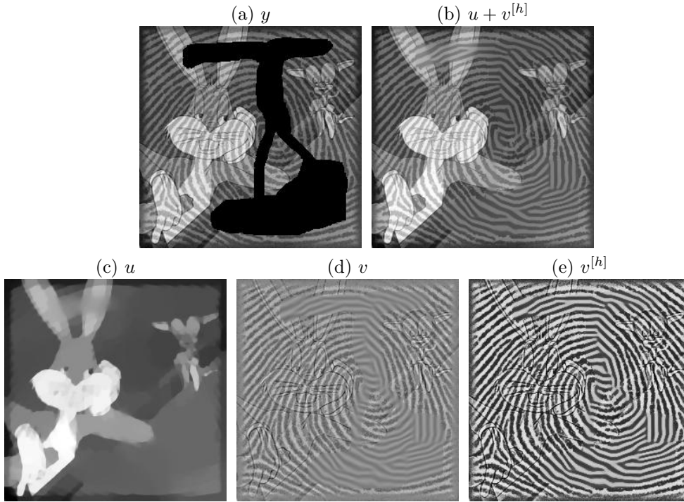
FIG. 6.5. (a) the image y to inpaint (the missing part is in black), the original image is f_0 in Fig. 5.4 ; (b) the reconstruction u + v^{[h]} using our non convex method ; (c) the inpainted geometric component u , (d) the sinusoidal approximation v of the texture component, (e) the inpainted texture component v^{[h]} after the change of contrast.
