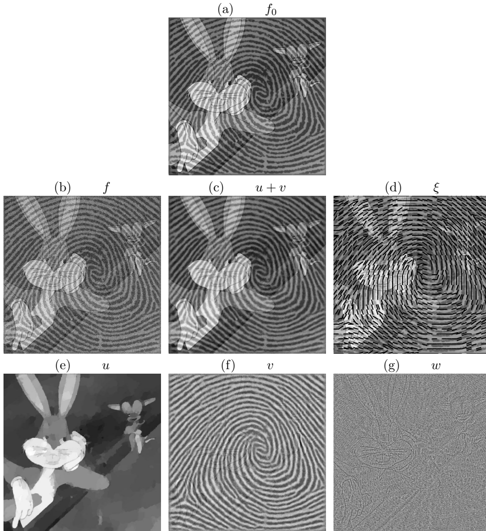
FIG. 5.4. (a) the original noise free image ; (b) the input noisy image f ; (c) the restored image u + v ; (d) the estimated orientations of oscillating patterns \xi ; (e) the sketch u of the image ; (f) the texture content v ; (g) the noise w .
