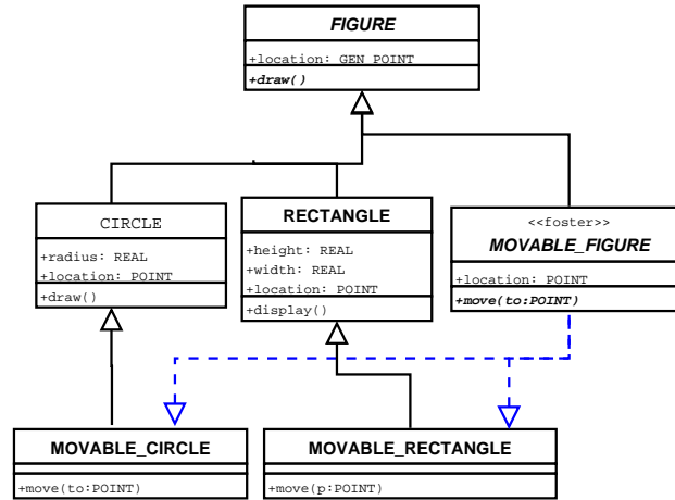
Fig. 5: Class diagram for Figure 4
