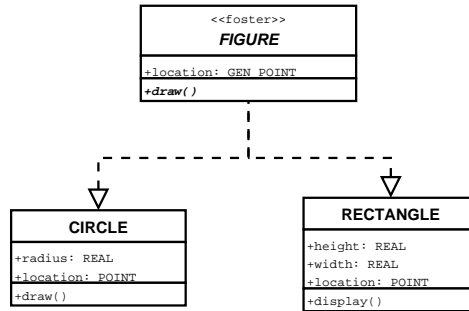
Fig. 3: Class diagram for Figure 2
