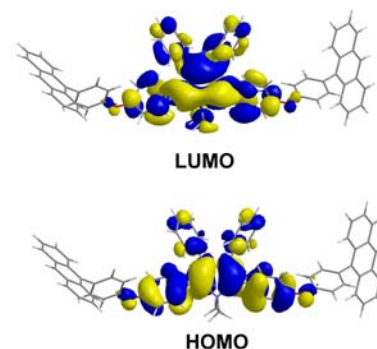
Figure 6. B3LYP/6-31G*-calculated HOMO and LUMO molecular orbitals for silole B' .
