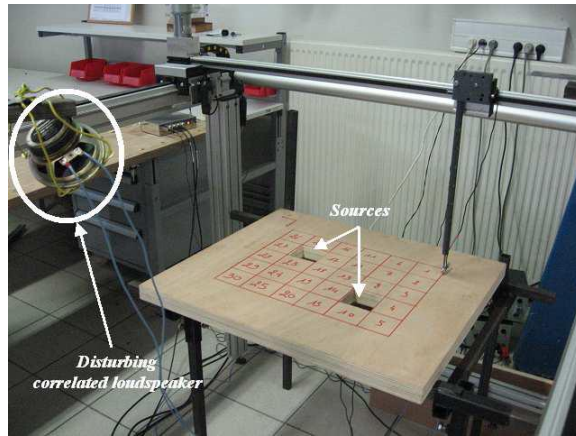
Figure 5. Location of the disturbing loudspeaker towards the measurement area
