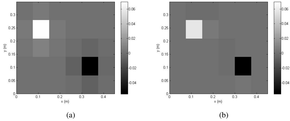
Figure 4: Comparison between (a) the reference map measured at 5 mm from the source and (b) the identification map obtained experimentally with the iPTF method at 240 Hz for a 450 \times 350 \times 20 mm virtual cavity
