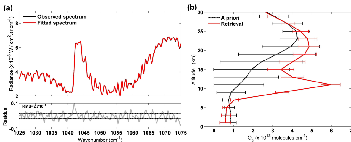
Fig. 5. (a) Spectral fit and residual for a IASI measurement made on 15 February 2008 in the eastern Atlantic (34.8° N, -29.3° E); the black lines at \pm 20 \text{ nW}/(\text{cm}^2 \text{ sr cm}^{-1}) correspond to the IASI radiometric noise value used to constrain this retrieval. (b) Associated retrieved (red) and a priori (black) ozone profiles in number density units.
