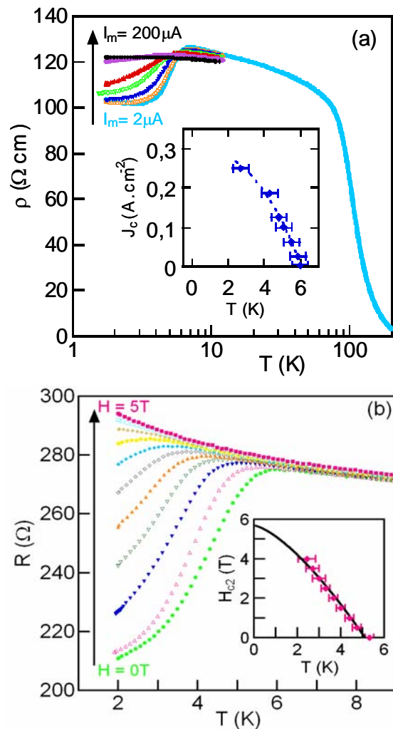
Figure 4. Critical current and critical field dependences of the resistivity (a) Low bias current evolution (from 2 to 200 \mu A) of the resistivity of sample #3 obtained with a 4 probes technique. The critical current density dependence of T_C is shown in the inset. (b) Low bias resistance of sample #4 measured at different magnetic fields. Inset: temperature dependence of the upper critical field.
