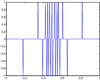
Figure 4: Control u_1^\varepsilon ( \varepsilon = 0.01 )
