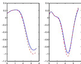
Figure 2: Adjoint vector
