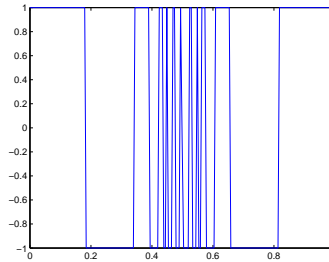
Figure 5: Control u_2^\varepsilon ( \varepsilon = 0.01 )
