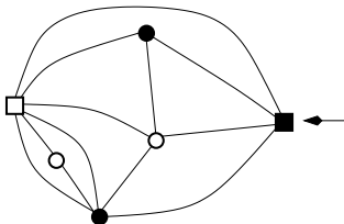
FIGURE 1. A (rooted) triangulation of the sphere, properly colored with 4 colors.
