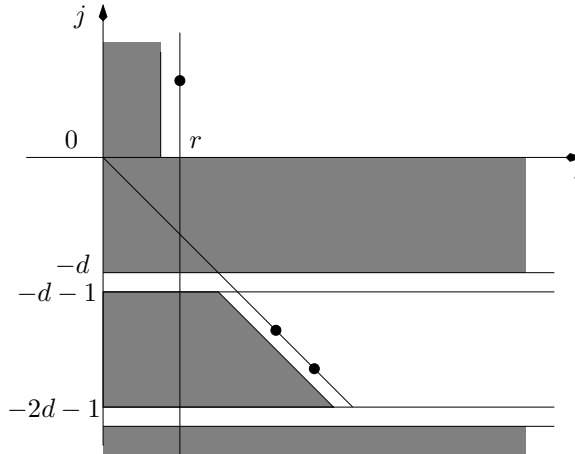
FIGURE 8. The coefficients g_{i,j} of G(y) . If (i, j) lies in one of the shaded areas, then g_{i,j} = 0 . The dots indicate non-zero coefficients.
