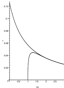
FIGURE 9. The curves P_2(\nu, \rho) = 0 (top) and P_1(\nu, \rho) = 1 (bottom), for \nu \in [0, 3] . The two curves meet at \nu_c \simeq 2.618 . Beyond this value, the curve P_1 is above P_2 (although very close at this scale). For every \nu , the radius is given by the highest of the curves.
