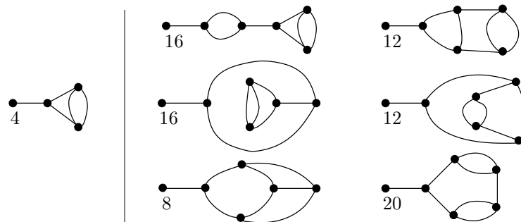
FIGURE 12. The loopless near-cubic maps with root-degree 1 and 3 or 4 faces, and their number of proper 3-colorings (the color of the root is fixed). In each column, the first two maps correspond to the same graph.
