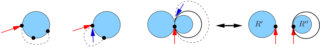
FIGURE 5. Decomposition of an incidence-marked map of Q'' .
