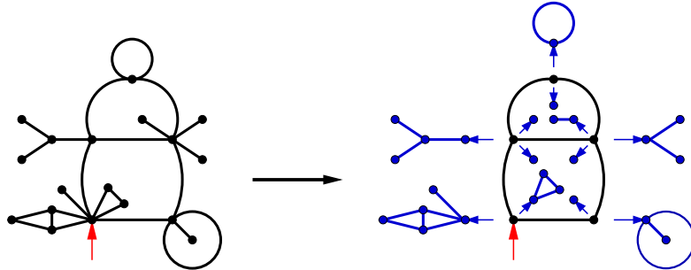
FIGURE 13. Decomposition of a map into a non-separable core in the corners of which are attached other maps.
