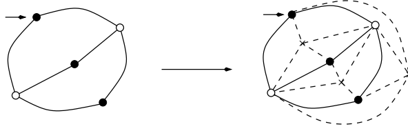
FIGURE 11. A bipartite map and the corresponding Eulerian triangulation.
