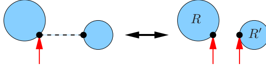
FIGURE 4. Decomposition of maps in Q' . The root-edge is dashed.
