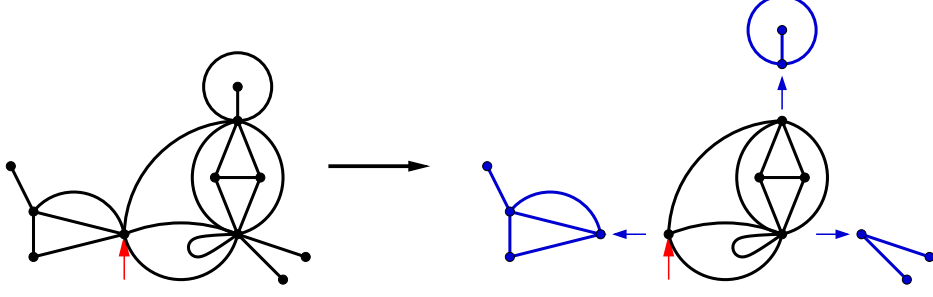
FIGURE 14. Decomposition of a map in \mathcal{Q} as a map in \mathcal{R} (containing the root-edge) to which are attached some maps in \mathcal{Q} .
