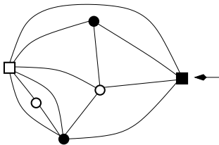
FIGURE 1. A (rooted) triangulation of the sphere, properly colored with 4 colors.
