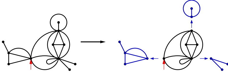
FIGURE 12. Decomposition of a map in \mathcal{Q} as a map in \mathcal{R} (containing the root-edge) to which are attached some maps in \mathcal{Q} .
