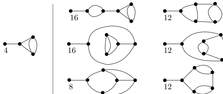
FIGURE 10. The loopless near-cubic maps with root-degree 1 and 3 or 4 faces, and their number of proper 3-colorings (the color of the root is fixed).
