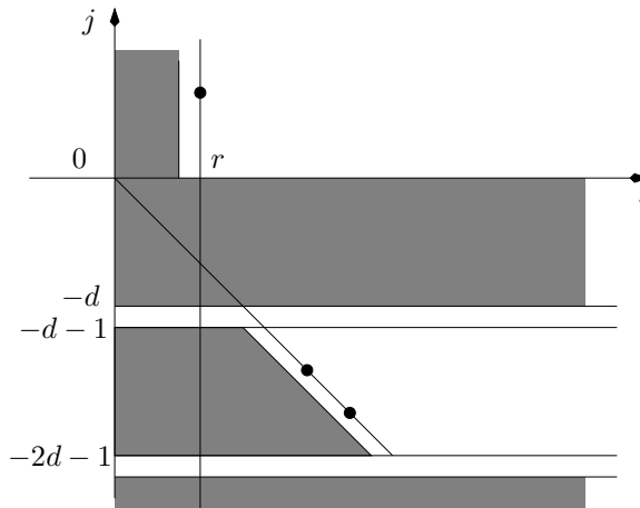
FIGURE 8. The coefficients k_{i,j} of K(y) . If (i, j) lies in one of the shaded areas, then k_{i,j} = 0 . The dots indicate non-zero coefficients.
