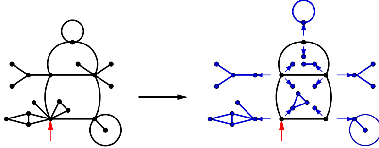
FIGURE 11. Decomposition of a map into a non-separable core in the corners of which are attached other maps.
