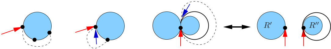
FIGURE 5. Decomposition of an incidence-marked map of \mathcal{Q}'' .
