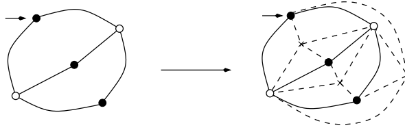
FIGURE 9. A bipartite map and the corresponding Eulerian triangulation.
