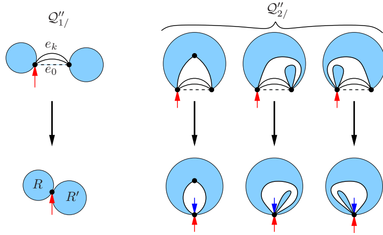
FIGURE 7. Top: the partition \mathcal{Q}''_{1/j} \uplus \mathcal{Q}''_{2/j} of the set \mathcal{Q}''_j . Bottom: the result of contracting the root-edge e_0 and subsequently removing the loops e_1, \dots, e_k .
