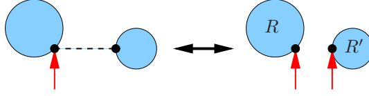
FIGURE 4. Decomposition of maps in \mathcal{Q}' . The root-edge is dashed.
