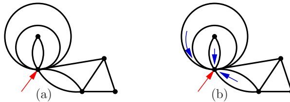
FIGURE 3. A map in \mathcal{Q} and one of the associated incidence-marked maps.
