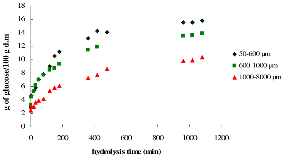
Figure 3. Kinetics of glucose production versus wheat straw particle size for unpretreated samples
