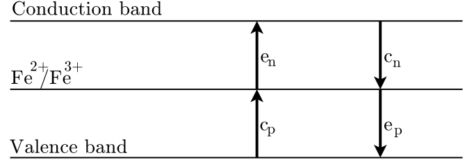
FIG. 1: Band transport two-carrier model with one middle band trap, characteristic, for instance, of Iron doped Indium Phosphide. The arrows show the electrons motions between the energy levels with the associated coefficient as in system (1) and expressions (2) and (3).
