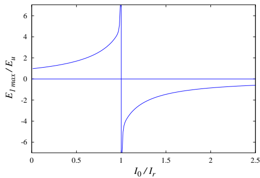
FIG. 6: The extremal value E_{1max}/E_u of the normalized space charge field vs the normalized background intensity I_0/I_r . The resonance at I_0 = I_r clearly appears.
