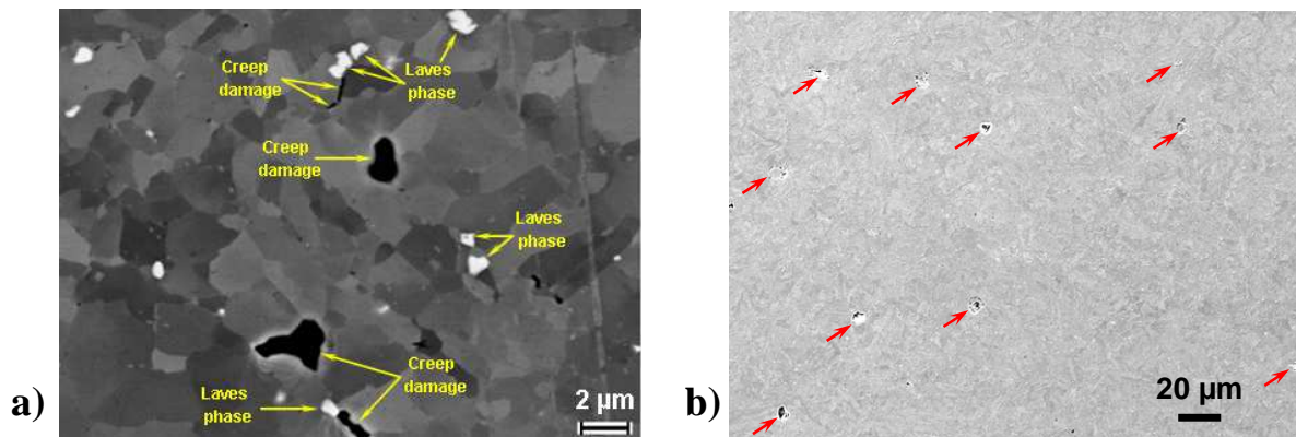
Figure 1 Creep damage in the P91 steel after creep at 600°C for 113,431h 7mm from fracture surface, SEM images, BSE-mode (a) and SE-mode (b)
