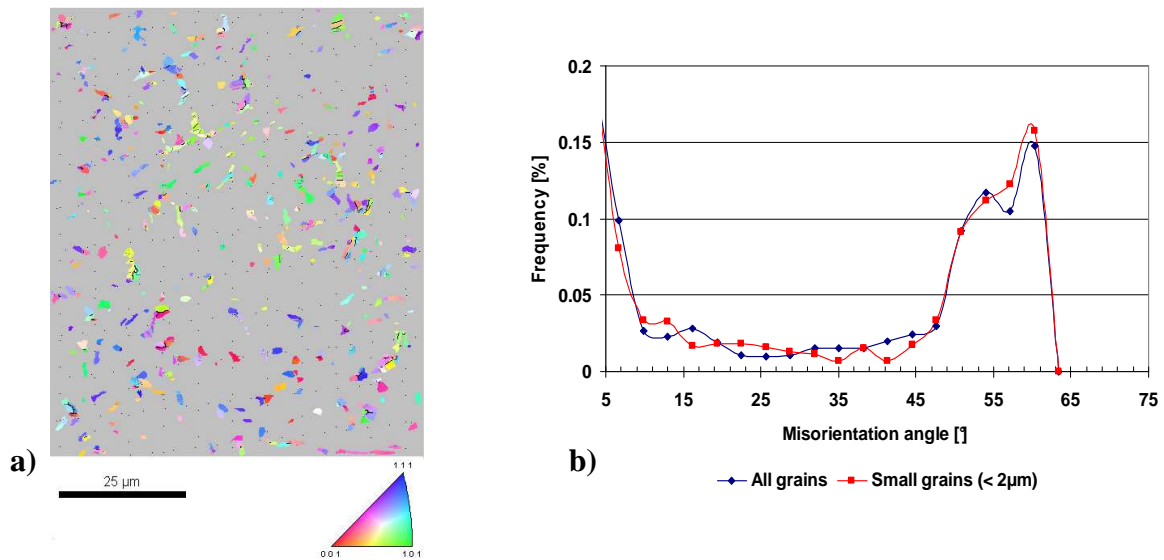
Figure 11 a) EBSD map of same area and same colour key as Figure 10a, showing only grains with a size lower than 2 μm; b) Comparison between misorientation angles for small grains and for the whole area
