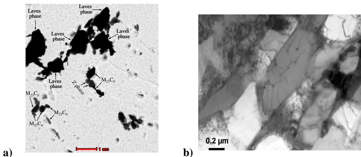
Figure 13 Microstructure of the steel after creep; a) extractive replica; b) thin foil
