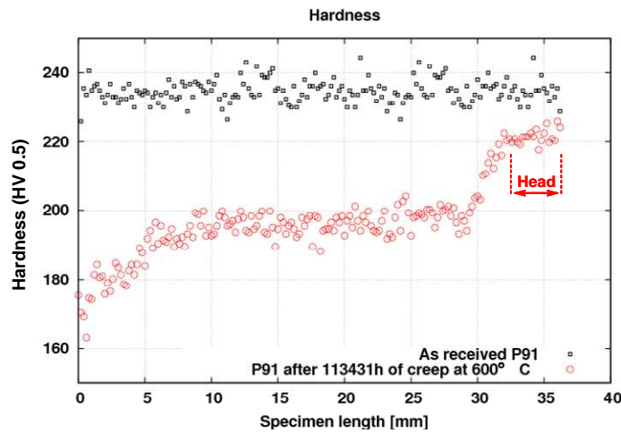
Figure 3 Evolution of hardness along the tensile direction of investigated creep specimen (circles) compared to that of a similar piece of as-received steel from the same pipe (squares)
