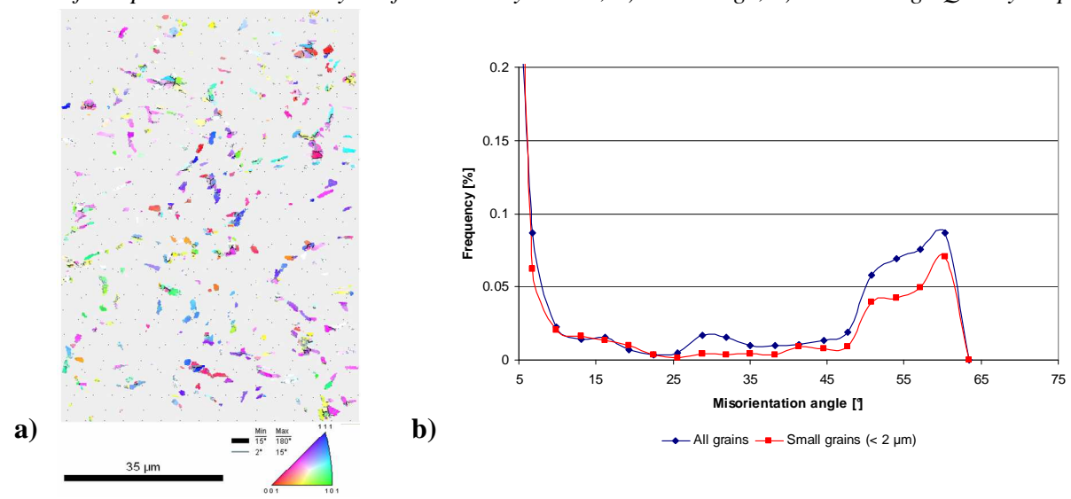
Figure 7 a) EBSD map of same area and same colour key as Figure 6a, showing only grains with a size lower than 2 µm; b) Comparison between misorientation angles for small grains and for the whole area
