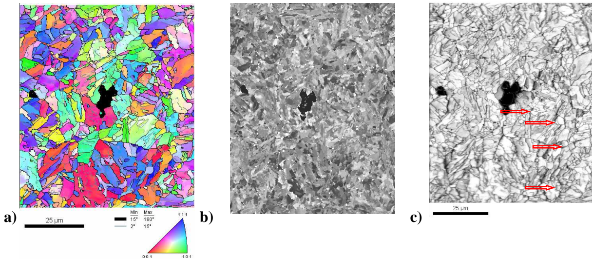
Figure 10 Microstructure of the P91 steel after creep (25mm from fracture surface). a) EBSD IPF (same colour key as in Figure 6a); b) BSE image; c) EBSD Image Quality map (some equiaxed subgrains are arrowed)
