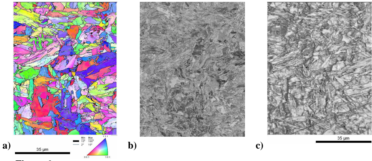
Figure 6 Microstructure of the as-received P91 steel. a) Inverse Pole Figure (IPF) with orientation of sample normal in the crystal frame as key colour; b) BSE image; c) EBSD Image Quality map
