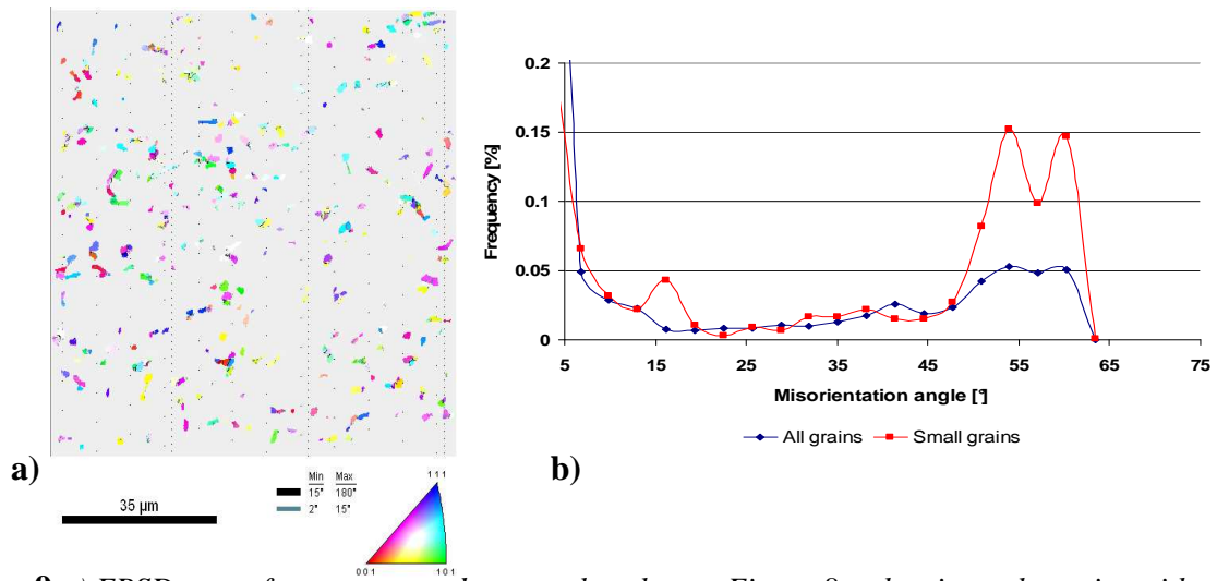
Figure 9 a) EBSD map of same area and same colour key as Figure 8a, showing only grains with a size lower than 2 μm; b) Comparison between misorientation angles for small grains and for the whole area
