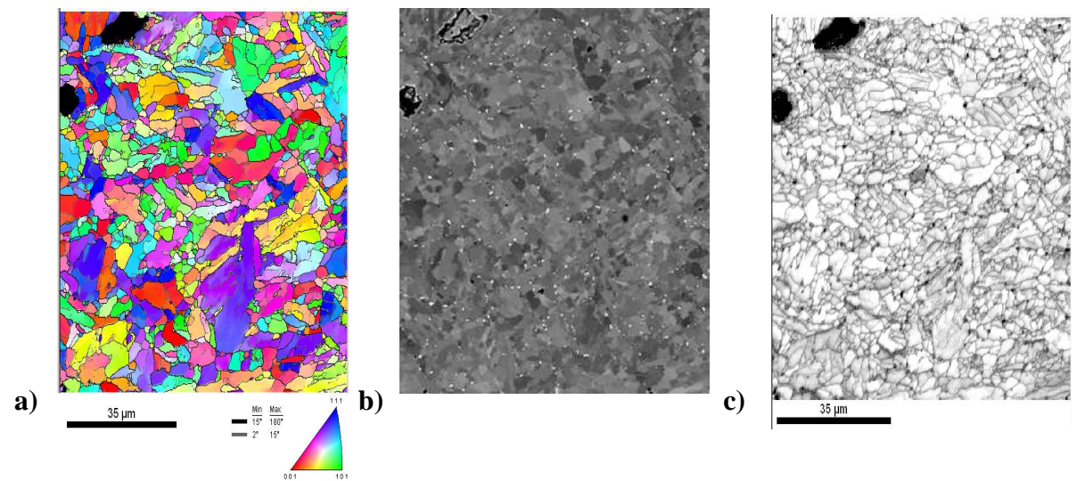
Figure 8 Microstructure of the P91 steel after creep (2mm from fracture surface) a) EBSD IPF (same colour key as in Figure 6a); b) BSE image; c) EBSD Image Quality map
