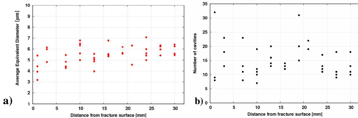
Figure 2 Average equivalent diameter (a) and number of cavities (b) calculated on areas of 342\mu\text{m}\times 214\mu\text{m} along the creep specimen axis
