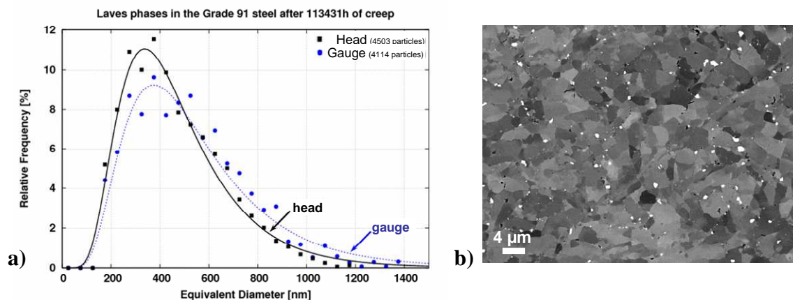
Figure 5 a) Size distribution of Laves phases in the P91 steel in the head (squares) and in the gauge portion (circles) of the creep specimen b) Microstructure of the P91 steel after creep, showing Laves phases (white)
