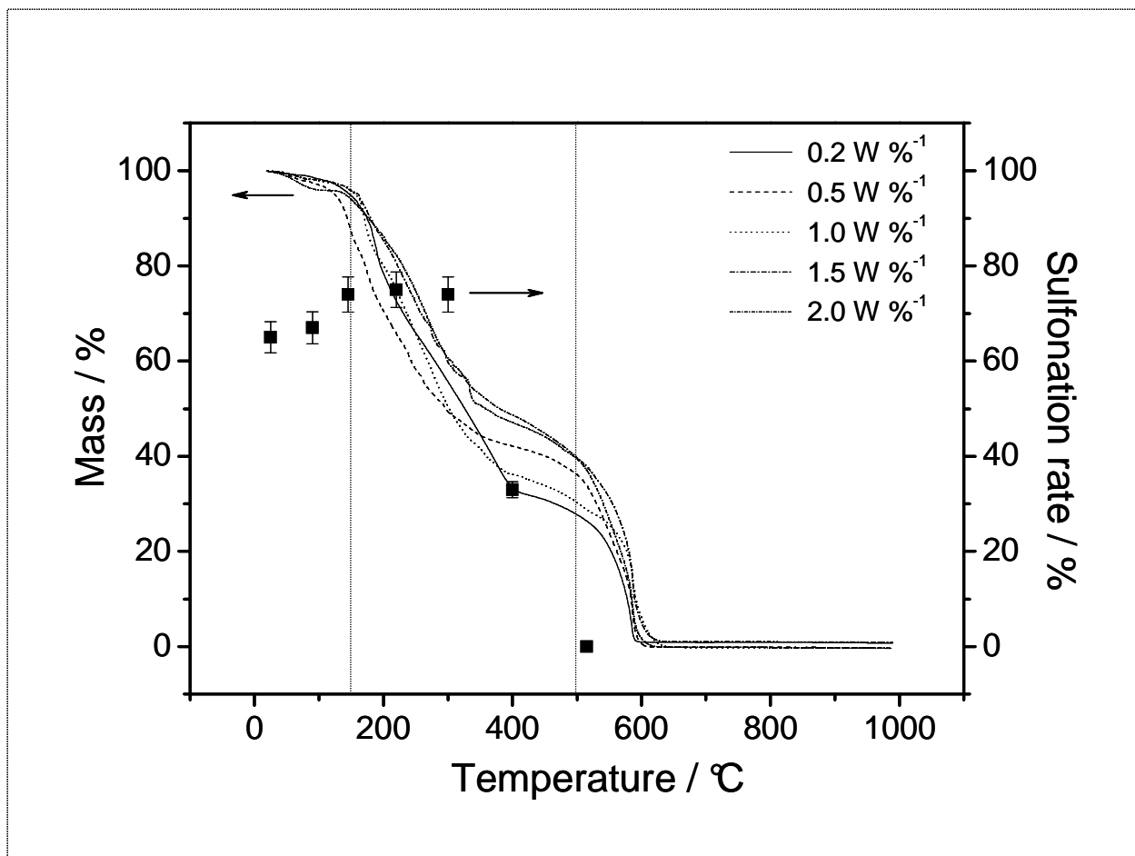
Figure 7: Thermogravimetric curves of plasma membranes deposited at different X values. For the membrane deposited at X = 0.5 \text{ W } \%^{-1} : sulfonation rate S_r at ambient temperature ( 25^\circ\text{C} ) and after heating at 90, 145, 220, 300, 400 and 515^\circ\text{C} .
