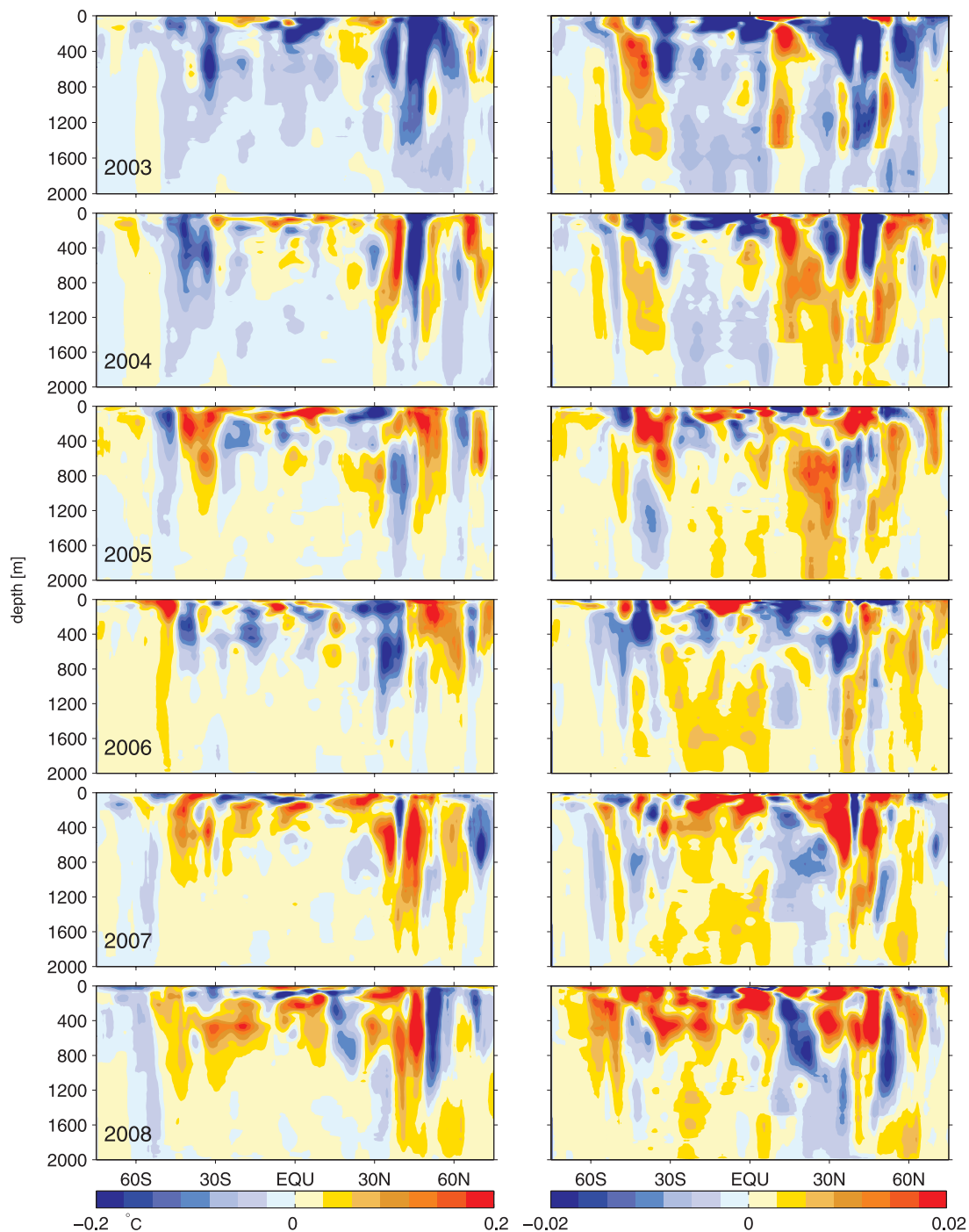
Figure 9. Same as Figure 8, but in the Atlantic basin.
