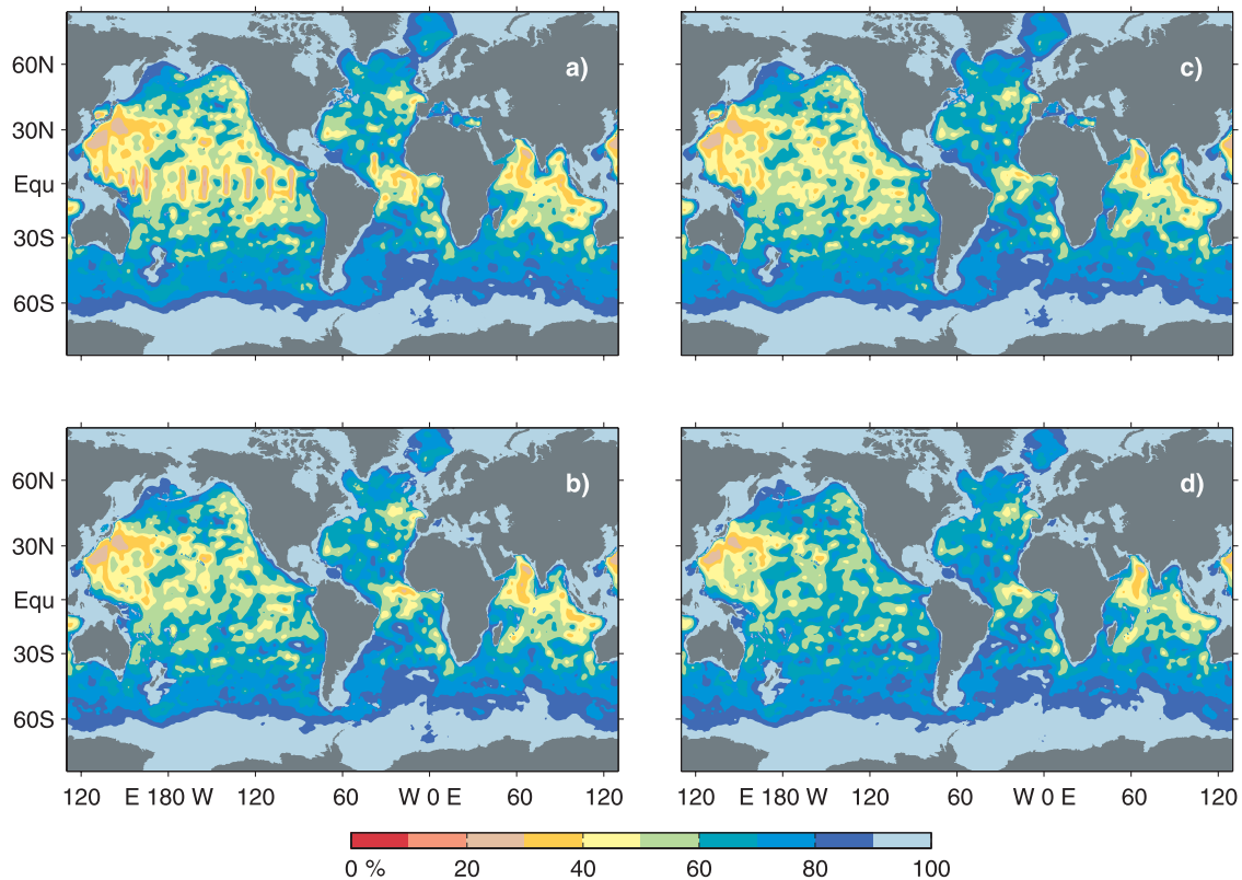
Figure 2. Horizontal map of percent of a priori variance for (a, b) temperature and (c, d) salinity measurements at 100 m (Figures 2a and 2c) and 1000 m (Figures 2b and 2d) depth. The statistic parameter is averaged in time during 2003–2008.
