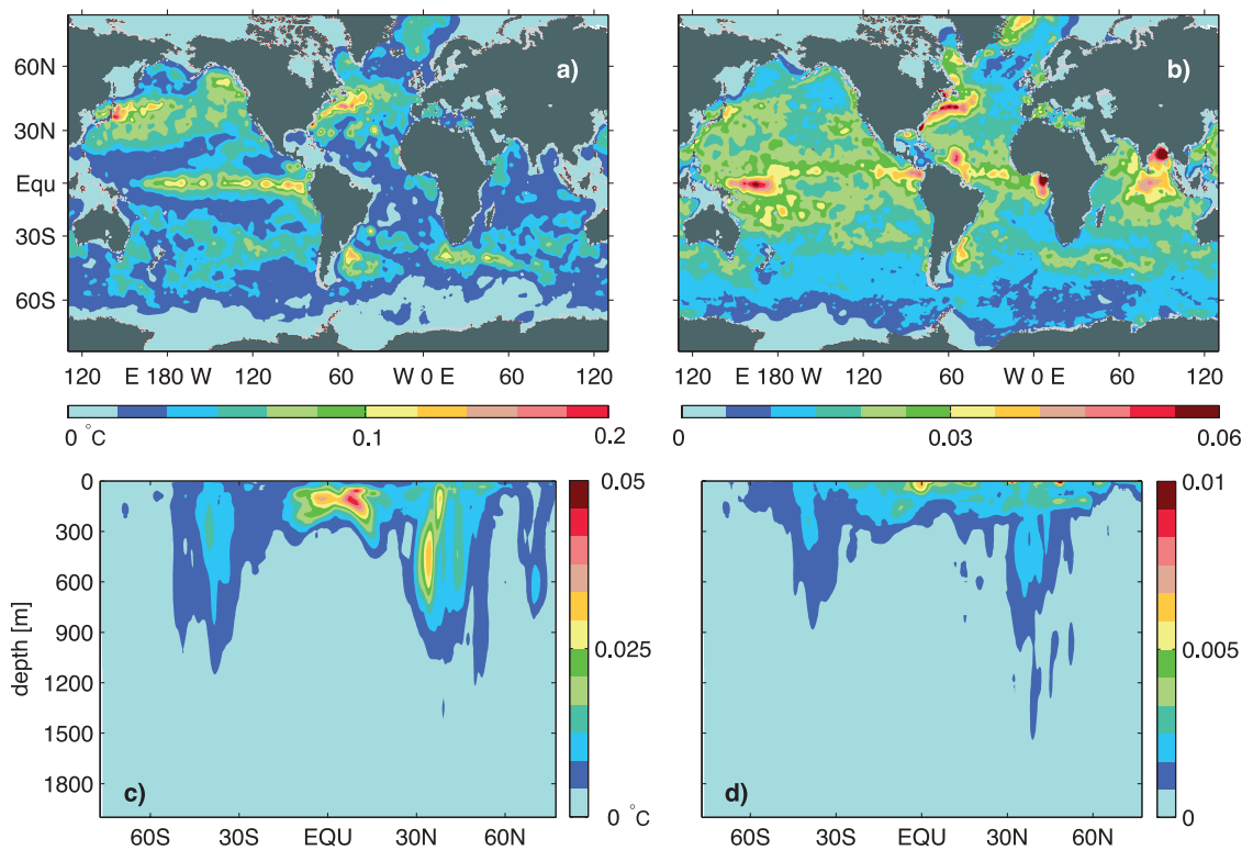
Figure 3. Error on the mean field over the period 2003–2008 of (a) temperature and (b) salinity at 10 m depth. One-dimensional (global zonal) mean of the error on yearly averaged (c) temperature and (d) salinity as a function of depth.
