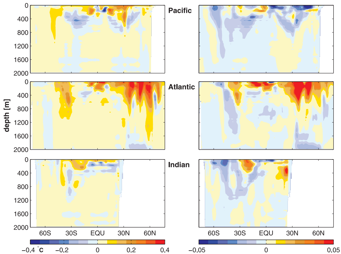
Figure 5. Basin-wide zonal averages of the difference field mean ARIVO anomaly (2003–2008) minus WOA05 for (left) temperature and (right) salinity at depth.
