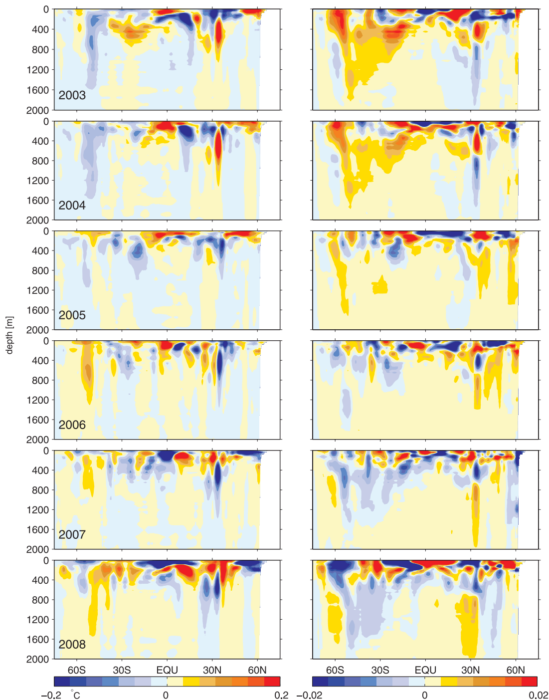
Figure 8. Yearly zonal average of (left) temperature and (right) salinity anomalies in the Pacific basin during 2003–2008 for the upper 2000 m depth.
