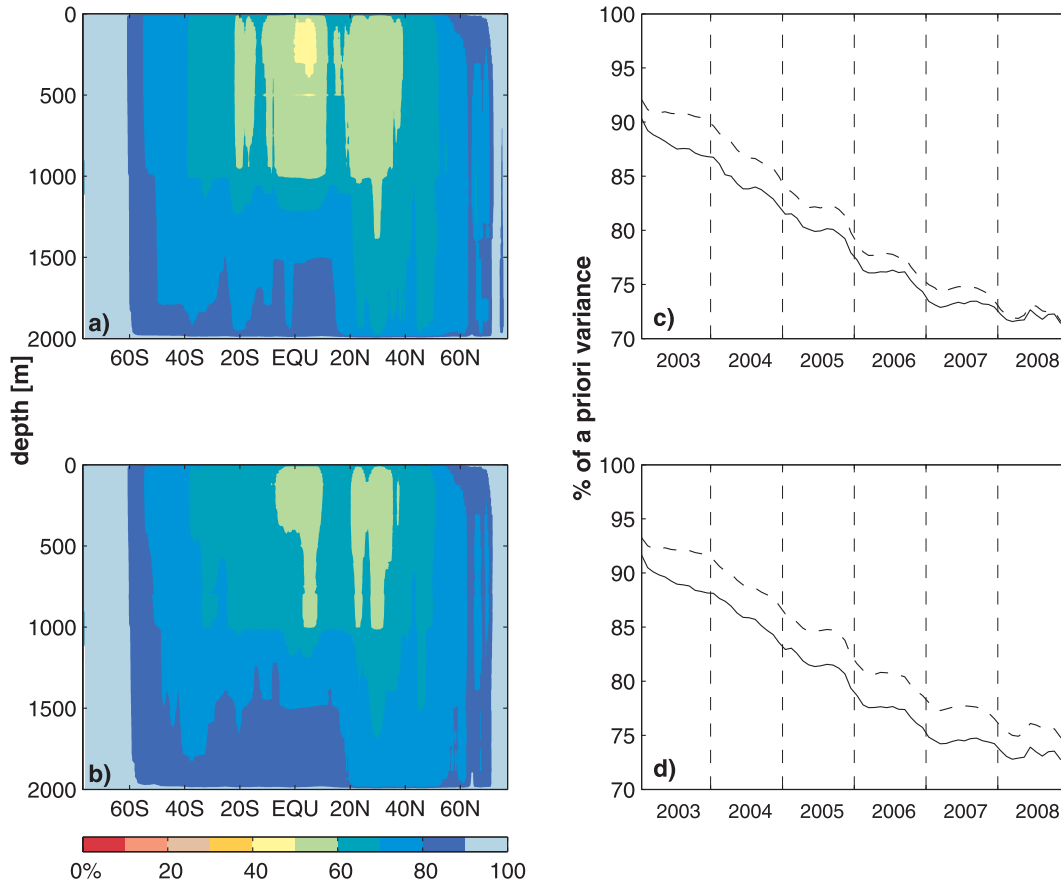
Figure 1. Global zonal average of percent of a priori variance represented for (a) temperature and (b) salinity. The statistic parameter is averaged in time during 2003–2008. Global zonal integral of a priori variance as a function of time for (c) temperature and (d) salinity, averaged over the upper 1000 m (bold line) and over the 1000–2000 m depth layer (dashed line). A 100% a priori variance indicates that no information is gained from the measurement field. EQU, equator.
