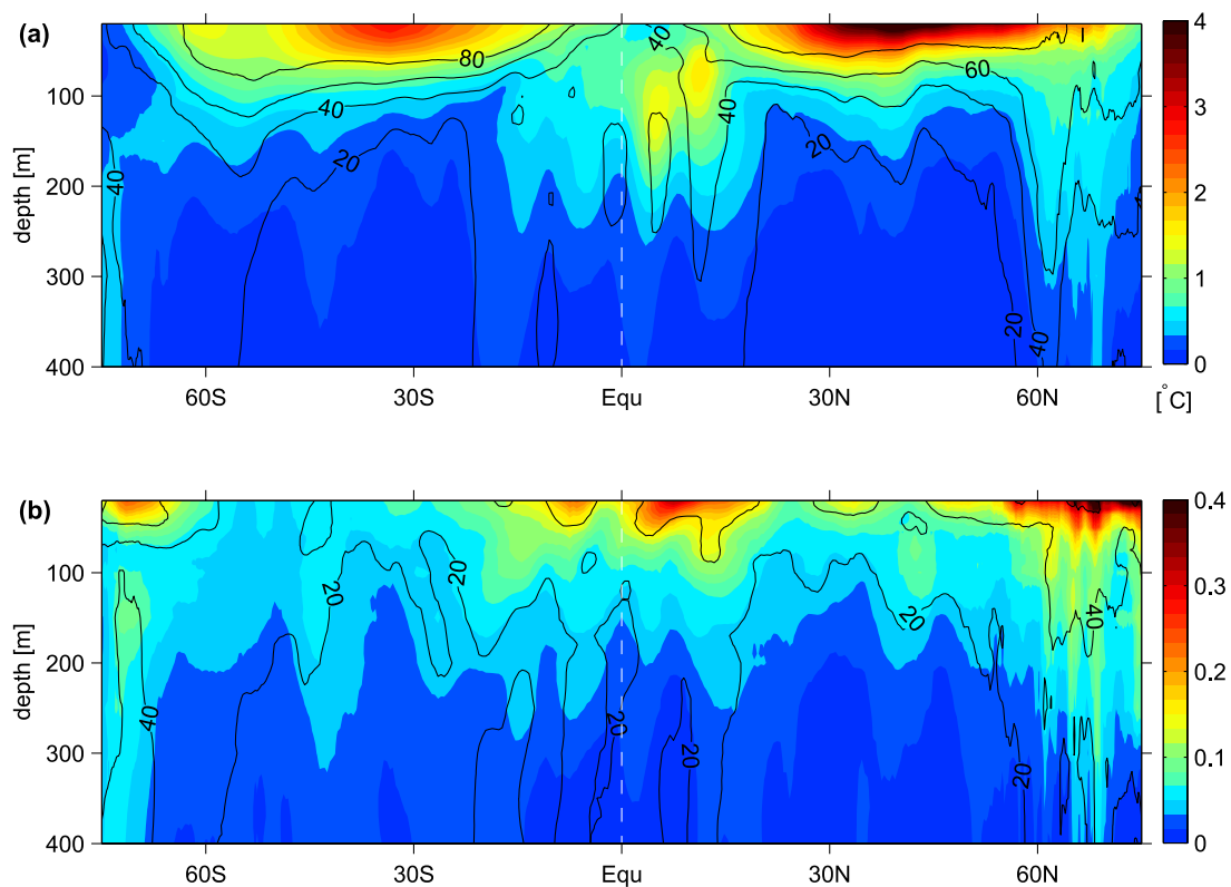
Figure 6. Global zonal average of the amplitude of the dominant harmonic of ARIVO (a) temperature and (b) salinity in the upper 400 m during 2003–2008. Contours show the variance in percent explained by the seasonal signal. White dashed lines indicate the equator.
