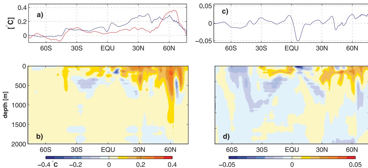
Figure 4. (a) Zonal average of the difference of National Oceanic and Atmospheric Administration optimum interpolation SST V2 of a short-term (2003–2008) mean minus a long-term (1990–2008) mean and of the ARIVO mean anomaly (2003–2008) minus WOA05a and WOA05b temperatures at 10 m depth (blue) together with (b) the distribution at depth of the latter difference field. (c) Zonal average of the difference field the ARIVO mean anomaly minus WOA05a and WOA05b salinities at 10 m depth and (d) its corresponding vertical distribution.
