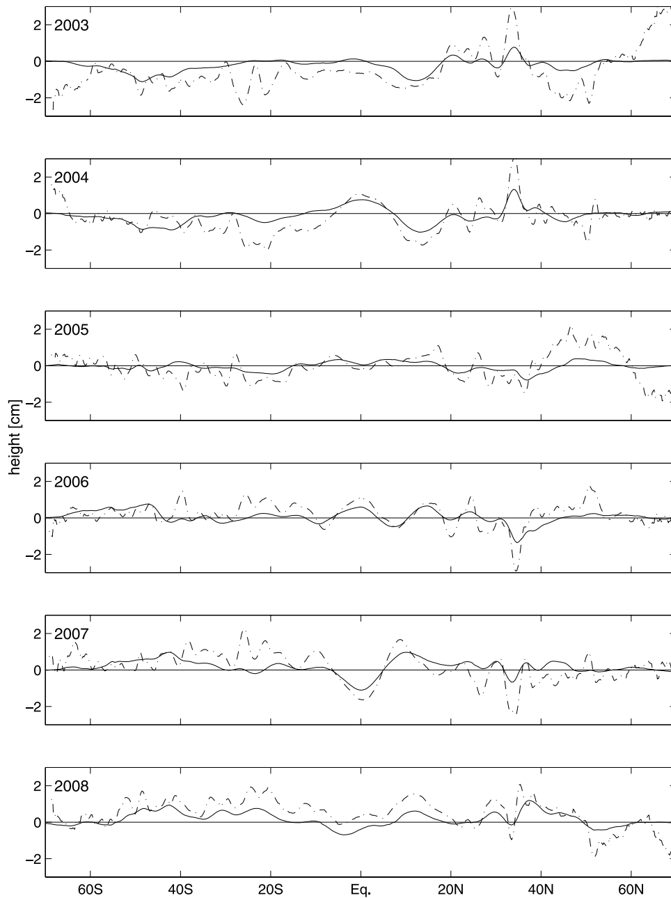
Figure 12. Yearly global zonal average of steric height (10–1500 m; solid line) and the corresponding satellite-derived sea level anomalies (www.aviso.oceanobs.com; dashed-dotted line) during 2003–2008 (note that only the first week of December 2008 was available in delayed mode).
