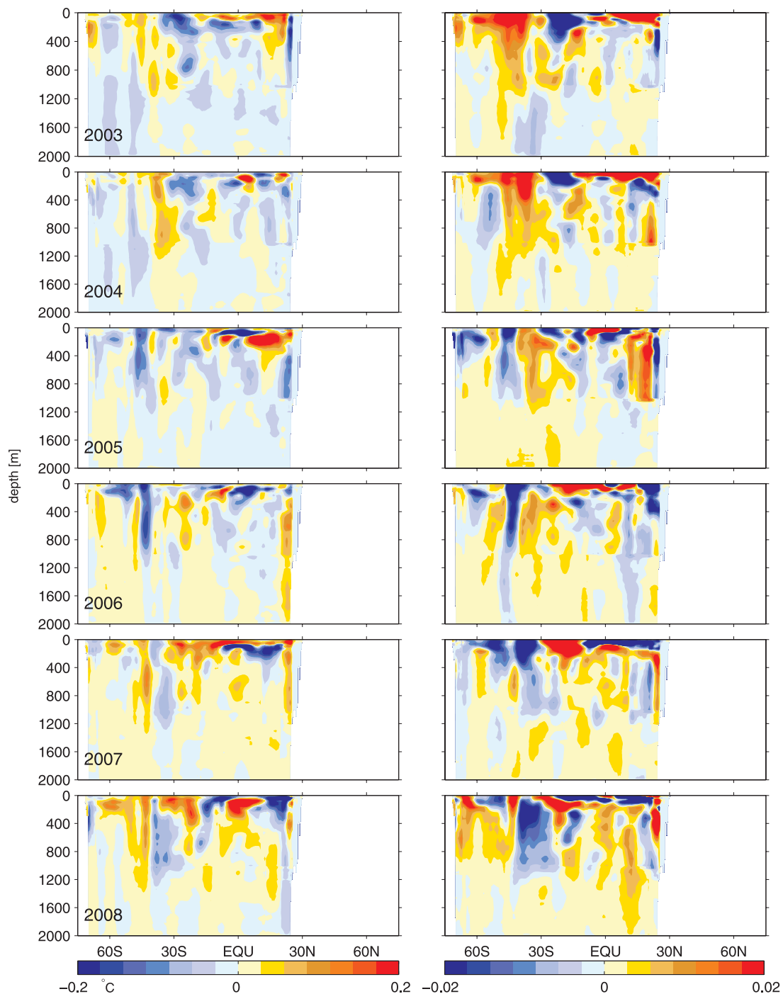
Figure 10. Same as Figure 8, but in the Indian basin.
