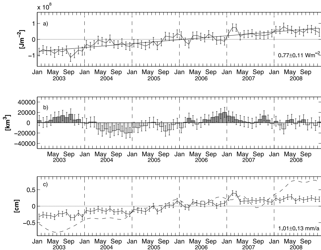
Figure 11. Time series of global mean (a) heat storage (0–2000 m), (b) freshwater content (0–2000 m), and (c) steric height (10–1500 m). The global mean sea level as measured by satellite altimetry ( http://www.aviso.oceanobs.com/msl ) is added in Figure 11c with a dashed line.
