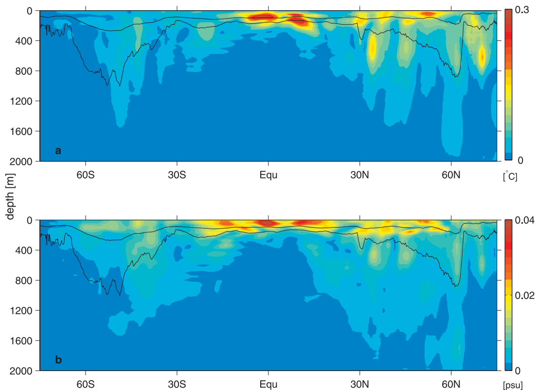
Figure 7. Global zonal averages of standard deviations of annual mean (a) temperature and (b) salinity derived from the ARIVO anomaly field 2003–2008 from the near-surface layer down to 2000 m depth. Mean and maximum pycnocline depths are added (black lines).
