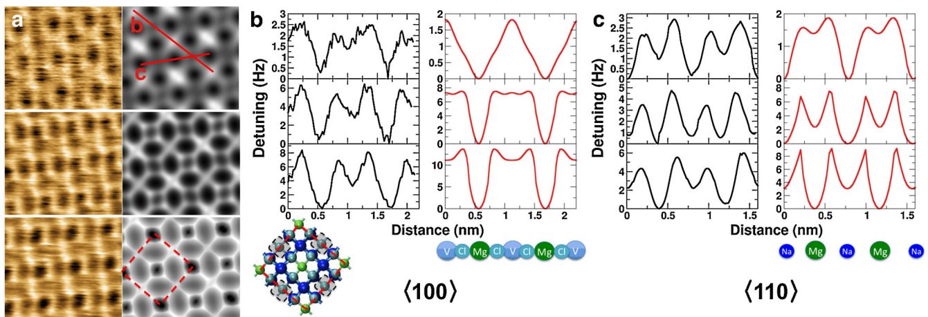
FIG. 2 (color online). Comparison of experimental and simulated data for NaCl: \text{Mg}^{2+} . The simulations used a Cl-terminated NaCl tip. (a) Images (color: experiment, gray: theory), (b) scan lines (red is simulated) in the \langle 100 \rangle direction, and (c) scan lines in the \langle 110 \rangle direction. The experimental data correspond to an average detuning of -16 , -22 , and -24 Hz (top-bottom, with a more negative detuning corresponding to imaging closer to the surface). The simulated data correspond to tip-surface heights of 0.45, 0.325, and 0.275 nm, resulting in average detunings of -16.4 , -21.8 , and -23.0 Hz, respectively.
