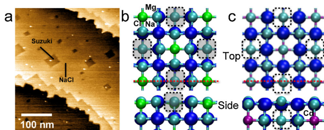
FIG. 1 (color online). (a) Topography image of Suzuki precipitates on the NaCl: Cd 2+ (001) surface. Atomic structure of the (b) Suzuki terminated NaCl: Mg 2+ surface and (c) NaCl-terminated NaCl: Cd 2+ surface. The shaded and unshaded boxes indicate surface and subsurface vacancy sites, respectively. The dashed line shows the plane of the side view.
