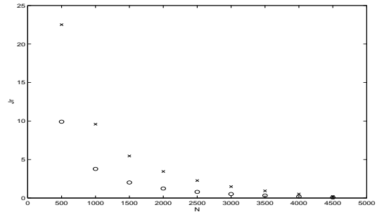
Fig. 3. Cost of the least costly experiment that satisfies Constraint 1 (circles) and of the white noise experiment that satisfies the same constraint (crosses), for different values of the data length.
