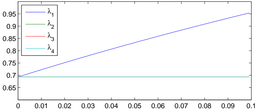
Figure 6: Lyapunov exponents evolution \epsilon_1 \in [0; 0.1] , \epsilon_2 = 4.10^{-5} , \epsilon_3 = 2.10^{-5} , \epsilon_4 = 10^{-5}
