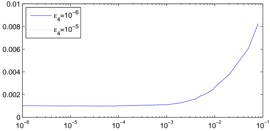
Figure 5: Distribution error evolution E_{c2} for \epsilon_1 \in [10^{-6}; 10^{-1}] , \epsilon_2 = 4\epsilon_4 and \epsilon_3 = 2\epsilon_4 for \epsilon_4 = 10^{-6} and \epsilon_4 = 10^{-5}
