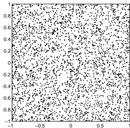
Figure 3: attractor in the phase plane (x_1; x_2)
