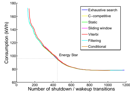
Figure 7: Consumption as a function of the number of shutdown transitions obtained with the different methods.
