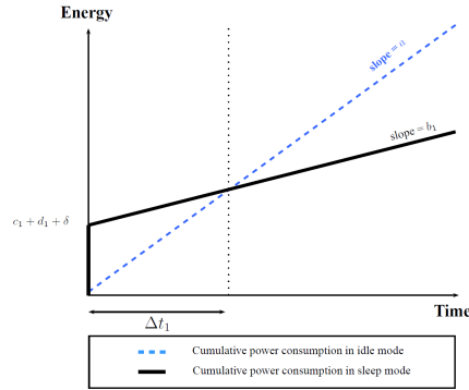
Figure 5: Graphical interpretation of \Delta t_1
