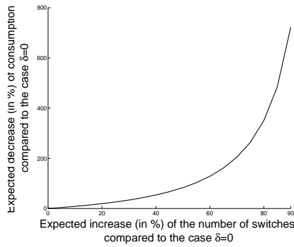
Figure 10: Expected decrease (in %) of the consumption as a function of the expected increase (in %) of the number of transitions. The reference model is a renewal process without penalty.
