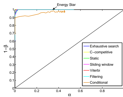
Figure 8: ROC curves obtained by varying the penalty \delta . Horizontally: type I error, vertically: 1 - type II error.
