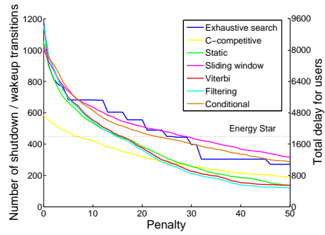
Figure 6: Number of shutdown transitions (left vertical axis) and total delay for users (right vertical axis) as the penalty \delta increases.
