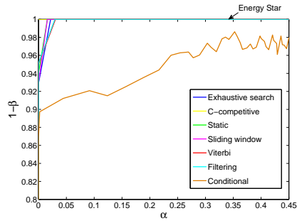
Figure 9: Close-up of upper left part of Figure 8 (ROC curves obtained by varying the penalty \delta ).
