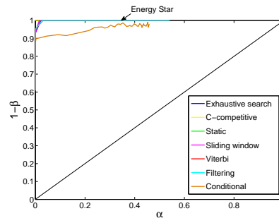
Figure 8: ROC curves obtained by varying the penalty \delta . Horizontally: type I error, vertically: 1 - \text{type II error} .
