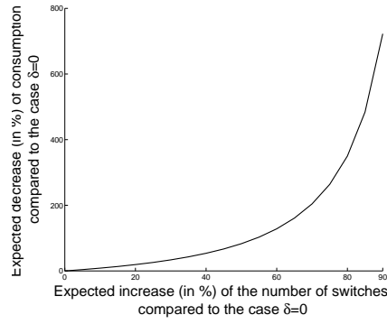
Figure 10: Expected decrease (in %) of the consumption as a function of the expected increase (in %) of the number of transitions. The reference model is a renewal process without penalty.
