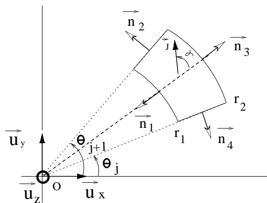
Figure 2. Parameters used for studying the magnetic field produced by the MRI structure
