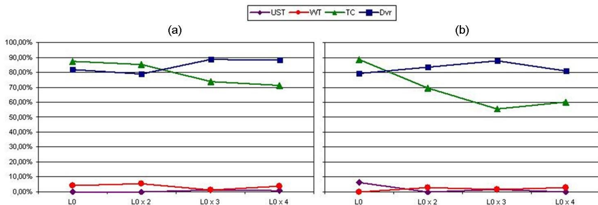
Figure 9: Proportions of broken rails detected by each detection system in respect of L_{TC} : (a) Reference value V=V_0 , (b) V=V_0 \times 2
