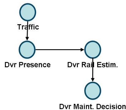
Figure 3: Bayesian Network modelling the diagnosis procedure of Metro drivers.
