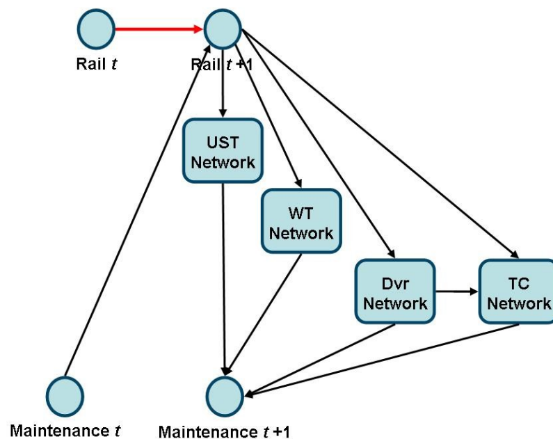
Figure 5: Dynamic bayesian network modelling the rail degradation, its diagnosis and the maintenance strategy.
