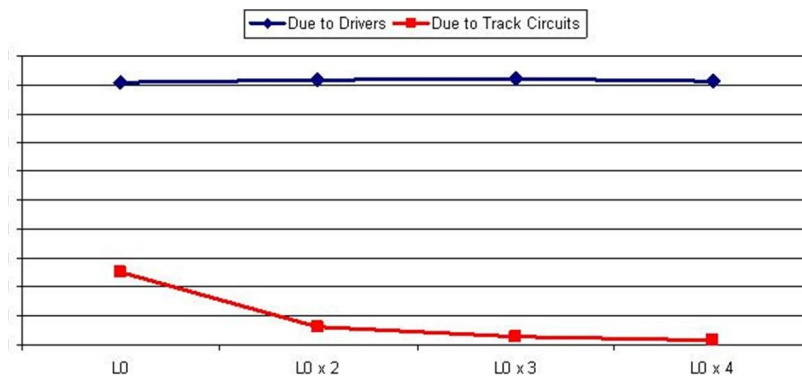
Figure 8: Influence of L_{TC} on false alarms.
