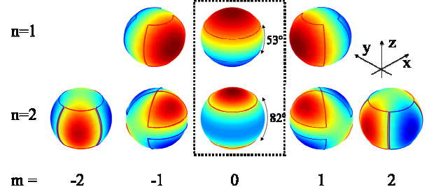
Fig. 2. 8 coils sensors for the identification of 1 and 2 orders. The flux is counted as positive for the red coils and negative for the blue ones
