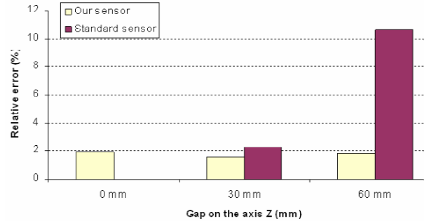
Fig. 5. Comparison between Standard and our sensor identifications: relative error compared to the actual and theoretical z -dipole with different gaps
