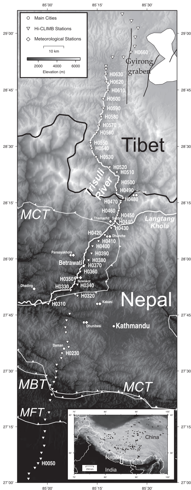
Figure 1. Location of the study area in central Nepal and southern Tibet. Main cities, Hi-CLIMB seismological stations as well as Department of Hydrology and Meteorology of Nepal (DHM) meteorological stations used in this study are represented by circles, inverse triangles, and diamonds, respectively. MCT, MBT, and MFT refer to Main Central Thrust, Main Boundary Thrust, and Main Frontal Thrust, respectively.
