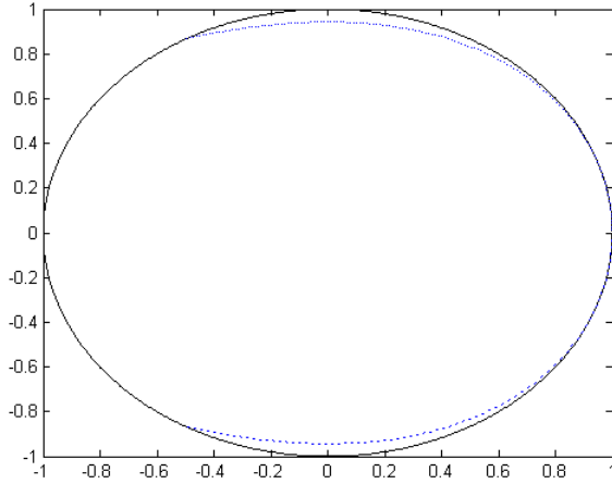
FIGURE 1. The curve \{\mathcal{A}(\kappa), \kappa \in \mathbb{S}^1\} (blue dots), and the unit circle (black line).
