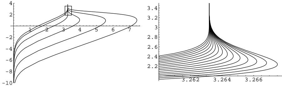
Fig. 2 Left: The set of all positive solutions of \Delta v_\sigma + \frac{\tau}{2} \xi \cdot \nabla v_\sigma + \sigma e^{v_\sigma} e^{-|\xi|^2/4} = 0 in C_0^2(\mathbb{R}^2) is now represented by the diagram s \mapsto (\log(1+M(s)), \log v_\sigma(0)) for \tau = 10^\alpha , \alpha = -2, -1, \dots, 3 . We observe that \max_{s \in \mathbb{R}} M(s) appears as an increasing function of \tau .
