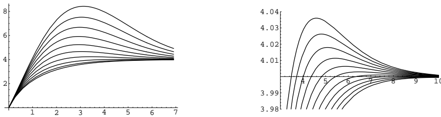
Fig. 5 Left: The value of mass \phi(\infty) = M(a, \tau)/(2\pi) in the logarithmic scale as a function of a , for \tau = 0.1 k^2 with k = 1, 2, \dots, 10 . Right: An enlargement around the value M(a, \tau)/(2\pi) = 4 in the logarithmic scale as a function of a , for \tau = 0.50, 0.55, 0.60, \dots, 1.00 .
