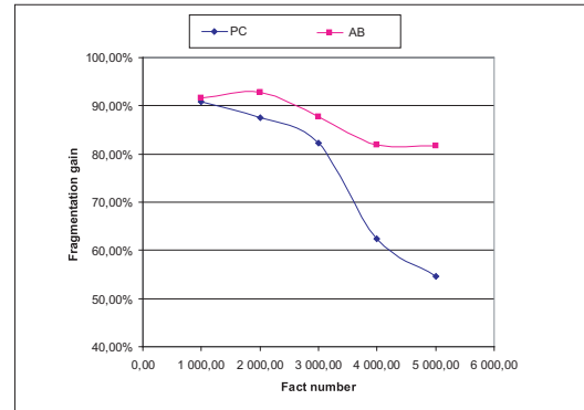
Figure 9: Fragmentation gain vs. warehouse size
