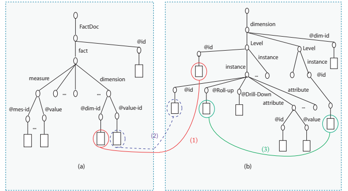
Figure 1: facts f .xml (a) and dimension d .xml (b) graph structure
