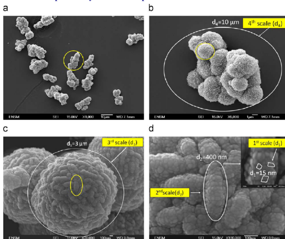
Fig 3: ZnS agglomerate morphology ( [TAA]=0.5\text{ mol L}^{-1} ; \text{pH}=1.5 ; [ZnSO_4]=0.025\text{ mol L}^{-1} ; T=80\text{ }^{\circ}\text{C} ; no stirring). (a) General view, (b) fourth scale, (c) third scale and (d) second and first scales.
