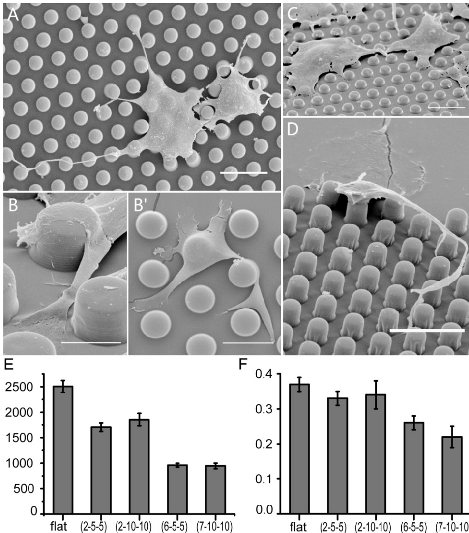
FIGURE 2 SEM pictures of 3T3 cells on the different types of pillars. (A) On (10-5-5) substrates, cells are mainly on the top of the pillars and present long protrusions (up to 60 \mu\text{m} ). (B and B') Cells are spread on the top and in between the pillars, occupying the whole spacing available on the (10-10-10) substrate. (C) Spread cells on (2-5-5) substrates present a morphology close to that observed on flat surfaces. (D) Cells at the interface between a flat substrate and a (6-5-5) micropillar substrate exhibit a change of morphology, with a large lamellipodium on the flat part and branched structures on the pillars. Scale bars = 20 \mu\text{m} . (E) Projected spreading area and (F) shape factor of 3T3 cells on flat (2-5-5), (2-10-10), (6-5-5), and (7-10-10) substrates.
