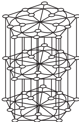
Figure 3: A pictorial representation of L_3 \times \text{GQ}(2,2) . In this representation the three doily-quads lie in three parallel planes and the 15 lines of type one, “tying” them together and lying fully in grid-quads, “penetrate” these planes perpendicularly.
