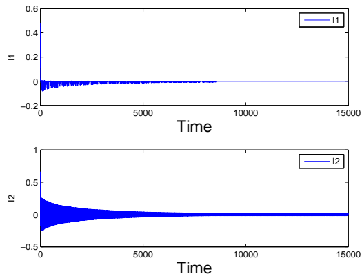
Figure 7. Time evolution of I_1 and I_2 ; system defined by (23) with feedback (12); |I_1| < \delta and |I_2| \leq C\delta .
