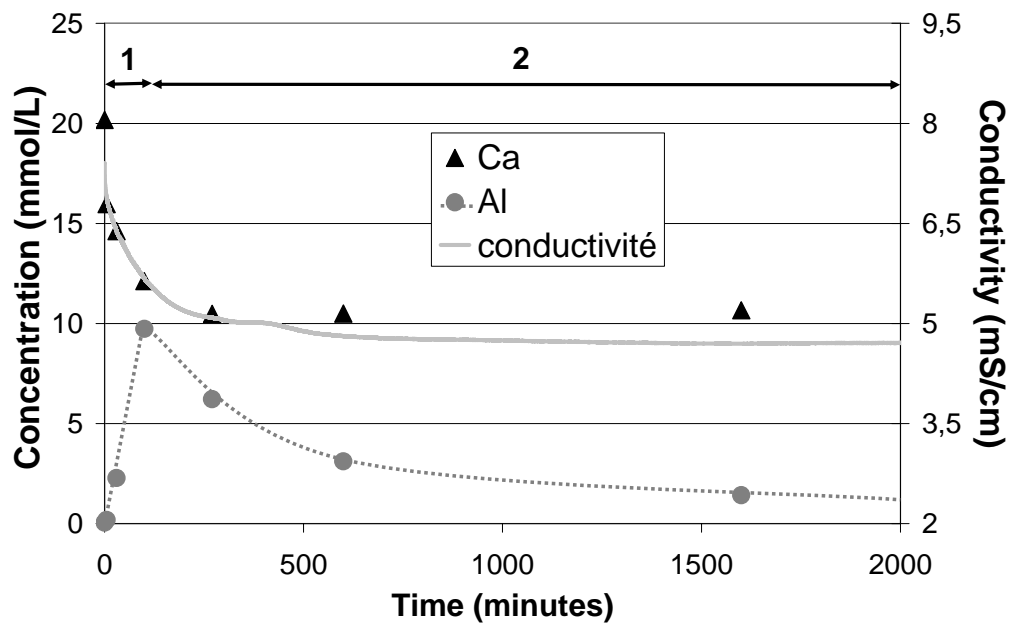
Figure 4. Impact of HEC H1 on C3A hydration in limewater without calcium sulphate: conductivity curve, calcium and aluminium concentration ( L/S = 20 , [Ca(OH)_2] = 20mM ).
