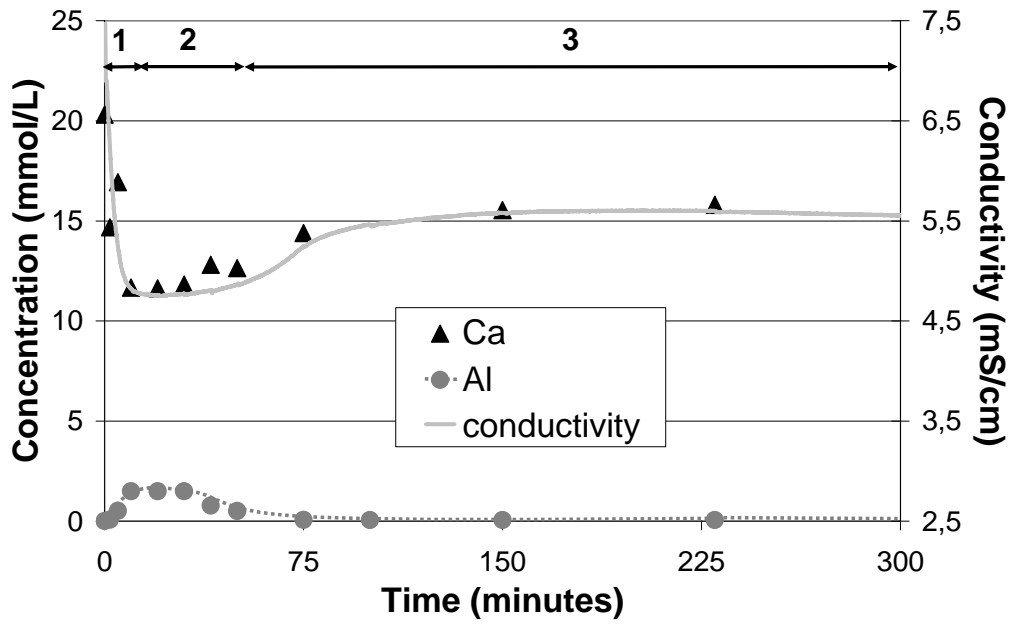
Figure 3. C3A hydration in limewater without calcium sulphate: conductivity curve, calcium and aluminium concentration ( L/S = 20 , [Ca(OH)_2] = 20mM ).
