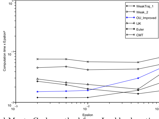
Figure 14: Multilevel Monte Carlo method for a Lookback option using different schemes.
