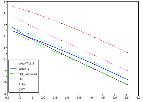
Figure 2: Strong convergence on the asset
