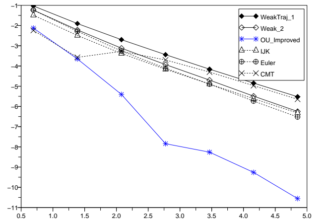
Figure 11: Illustration of the convergence rate for the Asian option
