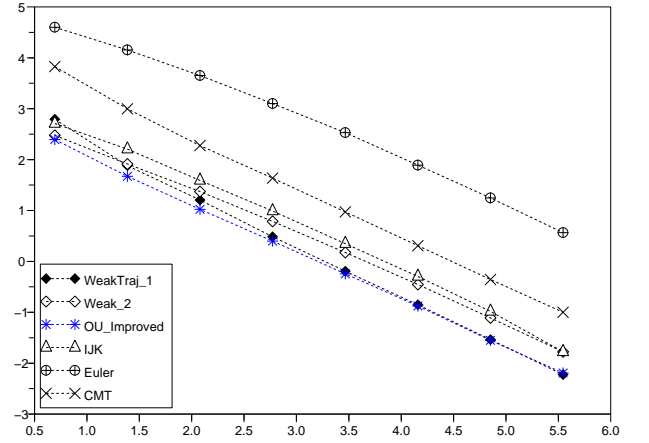
Figure 2: Strong convergence on the asset
