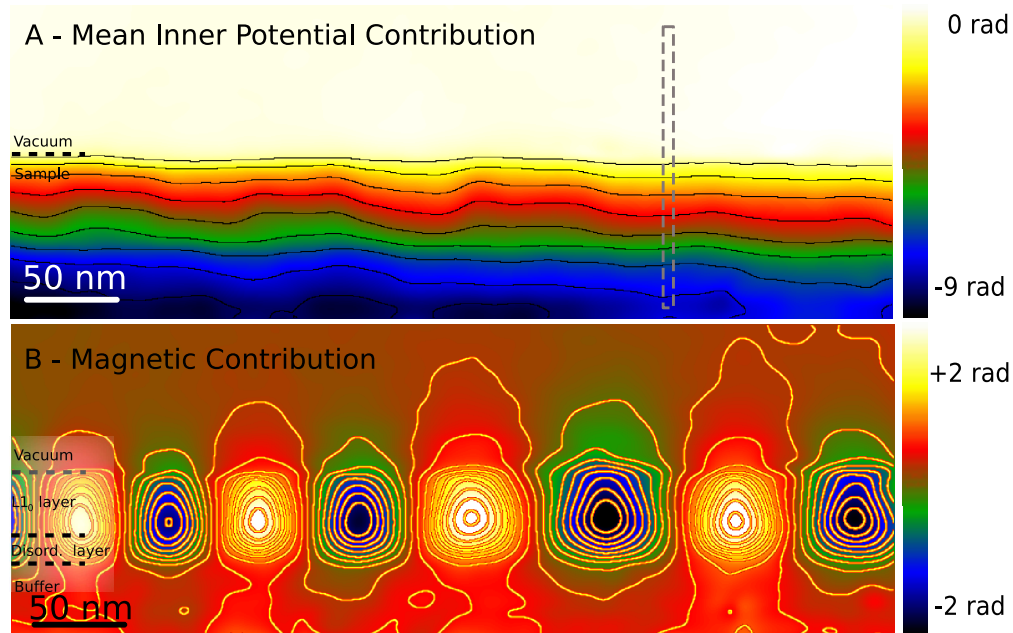
Figure 2: Mean Inner Potential (A) and magnetic (B) contribution to the phase of the electron wave. The color scale used here is a temperature scale described near each picture. The contour lines are for equi-phase lines and represent 1 radian for MIP contribution and 1/4 radian for magnetic contribution.
