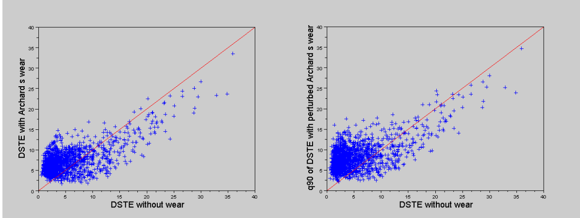
Figure 4: \Delta\text{STE} without wear vs. \Delta\text{STE} with Archard's wear profile ( \Delta\text{STE}_A , left), and vs. the 90% percentile of \Delta\text{STE} with randomly perturbed Archard's wear (right).
