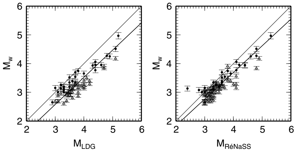
Figure 7. Comparison between moment magnitudes and local magnitudes. Pyrenees, black circles; Alps, gray triangles; One-to-one relationship, thin line; regression for the two data sets, solid line. Error bars are 1\sigma confidence level.
