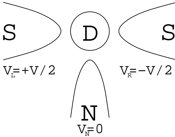
FIG. 1: Schematic picture of the setup. A single-level quantum dot is placed between two superconductors, which are biased with voltages \pm V/2 . An additional normal metal lead plays the role of a voltage probe 16 . Its coupling to the dot is controllable and its voltage is taken to satisfy a zero-current condition for the probe.
