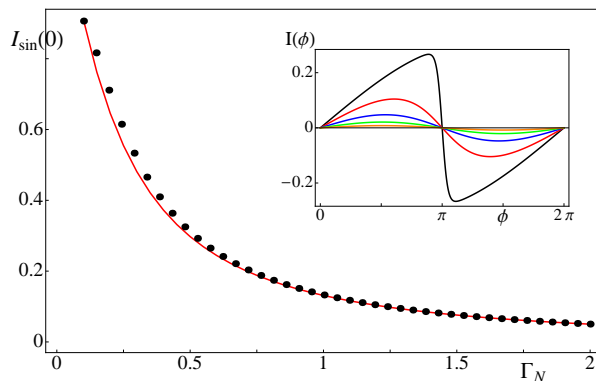
FIG. 5: Comparison between the first sine harmonic of the Josephson current J(\phi) (full curve) and the extrapolation at zero voltage of the first sine harmonic of the MAR current (circles). Inset: current phase relationship of the Josephson current for \Gamma_N = 0, 0.2, 0.5, 1.0, 2.0 (from larger to smaller amplitude). For both plots the parameters are \Gamma_S = 0.2 and \epsilon_0 = 0
