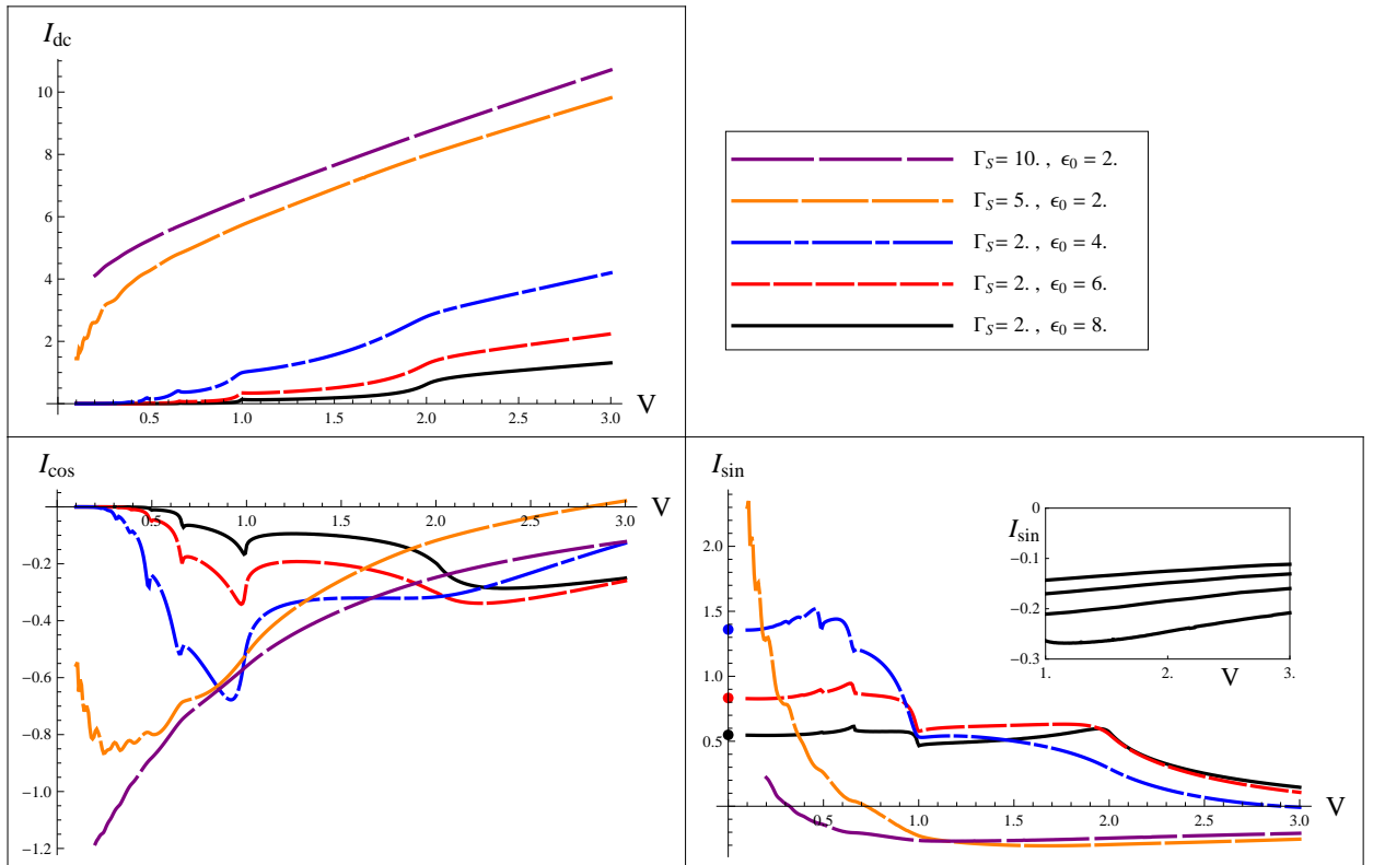
FIG. 2: Quantum Point Contact limit. DC (top panel), cosine first harmonic (lower left panel), and sine first harmonic (lower right panel) of the MAR current for different escape rates and dot level position. The circles on the y axis for the sine harmonic show the value of the first harmonics of the equilibrium Josephson current (computed independently). The inset in the sine harmonics panel shows results for \Gamma_S = 10, 20, 30, 40 (bottom to top) for V between 1.0 and 3.0.
