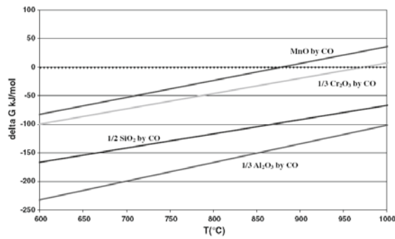
Figure 8: Standard free Gibbs energy of oxide formation [17] per mole O by H_2O or CO as a function of temperature under P_{CO} = 5 Pa , P_{H_2O} = 0.2 Pa , P_{H_2} = 20 Pa . The carbon transferred into the alloy by the reaction with CO is considered to be in equilibrium with Cr_{23}C_6 carbides formed in Haynes 230® [22]. Activities of elements are taken equal to their atomic fraction in Haynes 230® (ideal solution) except a_{Cr} which is taken approximately equal to 0.6 from activity measurements carried out on Haynes 230® [23]. The standard states of each element are defined by their most stable form at 1 bar and 298.15 K.
