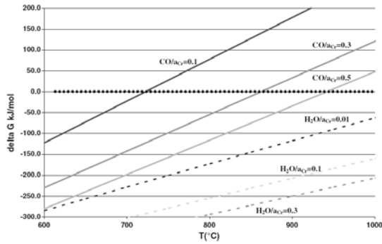
Figure 7: Standard free Gibbs Energy of formation [17] of Cr_2O_3 by H_2O or CO as a function of temperature and chromium activity in the alloy. P_{CO} = 5 Pa , P_{H_2O} = 0.2 Pa et P_{H_2} = 20 Pa .
