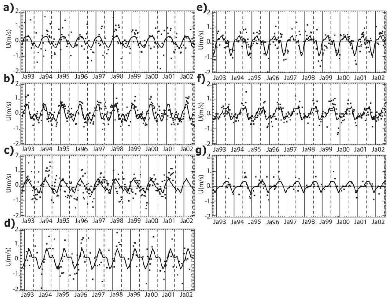
Figure 4. Evolution during 1992–2002 of the raw (unfiltered) altimetric cross-track geostrophic current anomaly for points (a) A, (b) B, (c) C, (d) D, (e) E, (f) F, and (g) G (dots). Superimposed on the raw current is the corresponding seasonal climatology (solid line) of the current anomaly (computed as a simple monthly average of the raw current time series). All currents are positive poleward (points A–F) and eastward (point G).
