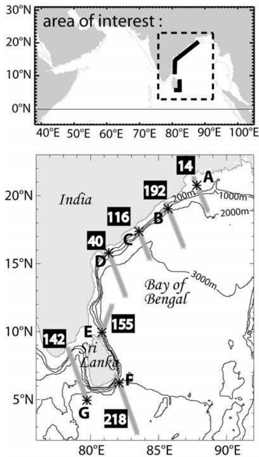
Figure 1. (top) The region of interest (north Indian Ocean) and the regime of the EICC. The thick lines show the axis along which the ship drifts (see Figure 2) are extracted and projected. (bottom) Layout of the T/P altimetric tracks portions used in the study (thick gray lines). Each T/P track is indicated in black squares. The position of the reference point of each track (points A, B, C, D, E, F, and G) used subsequently in the paper is marked with a black star. The 200 m, 1000 m, 2000 m, and 3000 m isobaths are shown. Bathymetry is from Sindhu et al. [2007].
