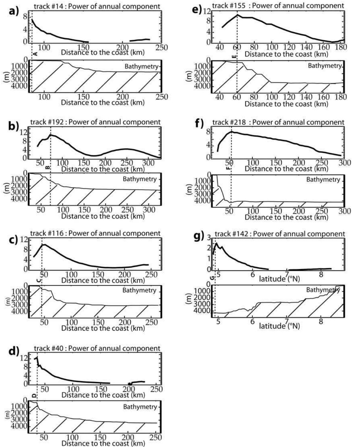
Figure 7. Nonnormalized Lomb periodograms of the annual variability of cross-track geostrophic current for all the tracks. The power of the annual component of the cross-track current is plotted (a, b, c, d, e, f) as a function of the position along the altimetric track and (g) as a function of latitude. Only the values exceeding the 95% significance levels are plotted. Below each periodogram, we present the bathymetry along the track (in m). Superimposed in dotted line are the positions of the reference points (A–G) along the tracks.
