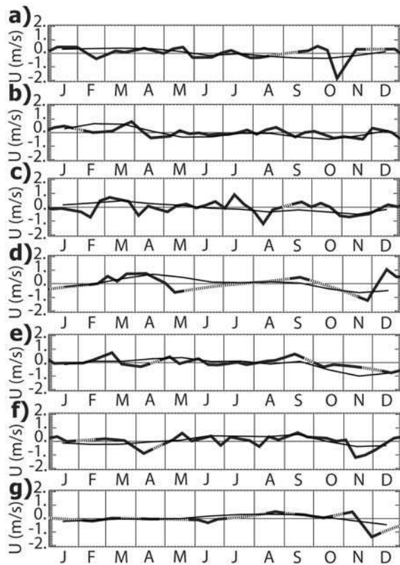
Figure 9. Evolution from January to December 1999 of the intraseasonal component of the altimetric cross-track geostrophic current anomaly (thick line) for EICC points (a) A, (b) B, (c) C, (d) D, (e) E, (f) F, and (g) G. The dotted portions show the gappy parts of the original (raw) time series. Superimposed (thin line) is the corresponding seasonal climatology. All currents are positive poleward (points A–F) and eastward (point G).
