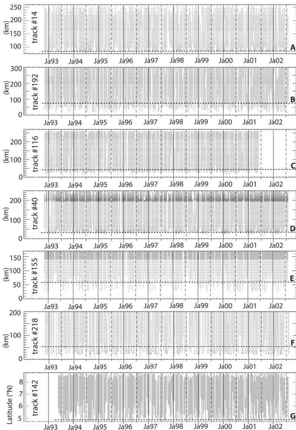
Figure 3. Data coverage of the cross-track geostrophic surface current anomaly for each track. It is plotted as a function of time (from November 1992 to July 2002). One thin vertical solid (dashed) line is drawn every 1 January (1 July). The position of each point along the track is defined as the distance (in km) from the point to the nearest shore (except for Track 142 located west of Sri Lanka, where it is plotted as a function of latitude). Superimposed (horizontal dotted lines) are the positions of the reference points (points A, B, C, D, E, F, and G; see Figure 1) along the tracks.
