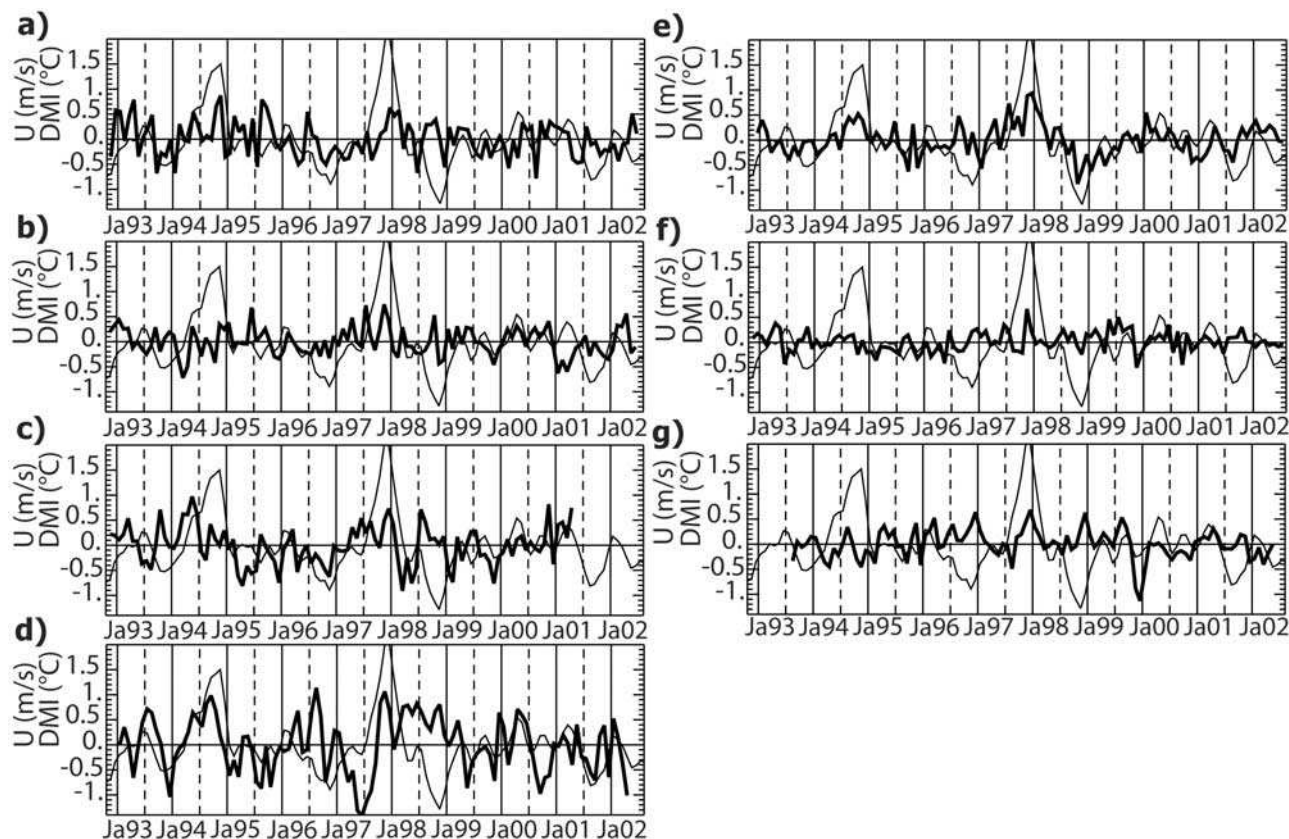
Figure 10. Evolution during 1992–2002 of the anomaly (with respect to the monthly climatology presented in Figure 6) of the altimetric cross-track geostrophic current anomaly (thick line) for EICC points (a) A, (b) B, (c) C, (d) D, (e) E, (f) F, and (g) G. All currents are positive poleward (points A–F) and eastward (point G). Superimposed (thin line) is the Dipole Mode Index time series (as defined by Saji et al. [1999]).
