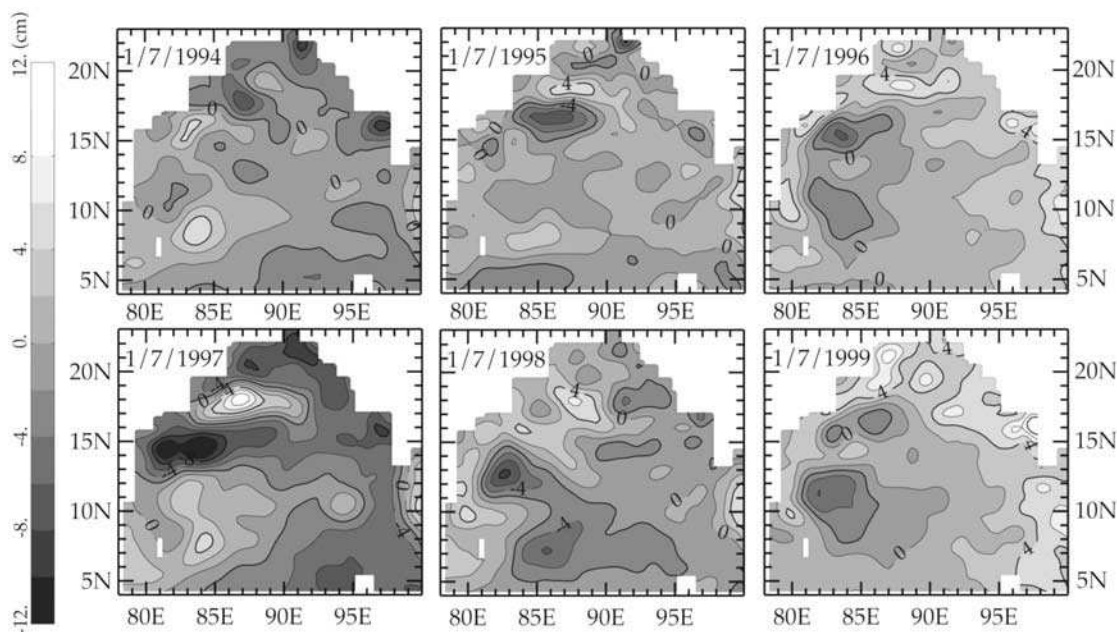
Figure 14. Low-passed (interannual) SLA for the Bay of Bengal from Archiving, Validation, and Interpretation of Satellite Oceanographic data [1996], plotted for some days from 1 July 1994 to 1 July 1999. The date is indicated. Contour interval is 2 cm.
