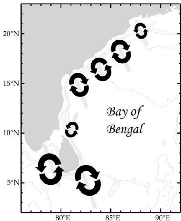
Figure 13. Schematic of the EICC circulation pathways. The recirculation cells are represented with arbitrary directions but with dimensions scaling like the anticorrelation length scales given by Figure 11.
