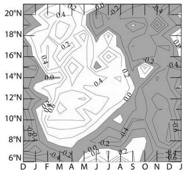
Figure 2. Seasonal climatology of EICC surface velocity as a function of latitude along Sri Lankan (6°N–8°N) and Indian (10°N–21°N) east coasts (inferred from Mariano et al. [1995]) ship drifts projected in the alongshore direction. Contour interval is 0.2 m s -1 . Positive values indicate eastward and northward current. Negative values are shaded.
