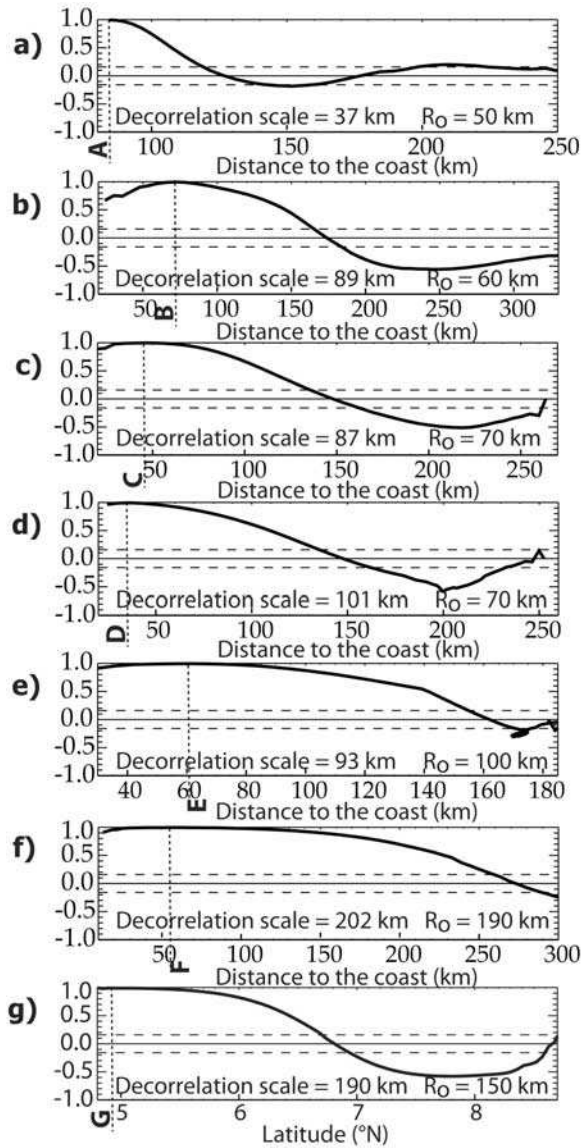
Figure 11. Correlation along each altimetric track of the cross-track geostrophic current anomaly with the reference point (A–G). The positions of the reference points are indicated by dotted lines, and the 95% significance level is indicated by dashed lines. The decorrelation scale (defined as the distance between the reference point and the first crossing of the 95% significance level) is indicated for each point, as is the value of R_o from Chelton et al. [1998] (in km).
