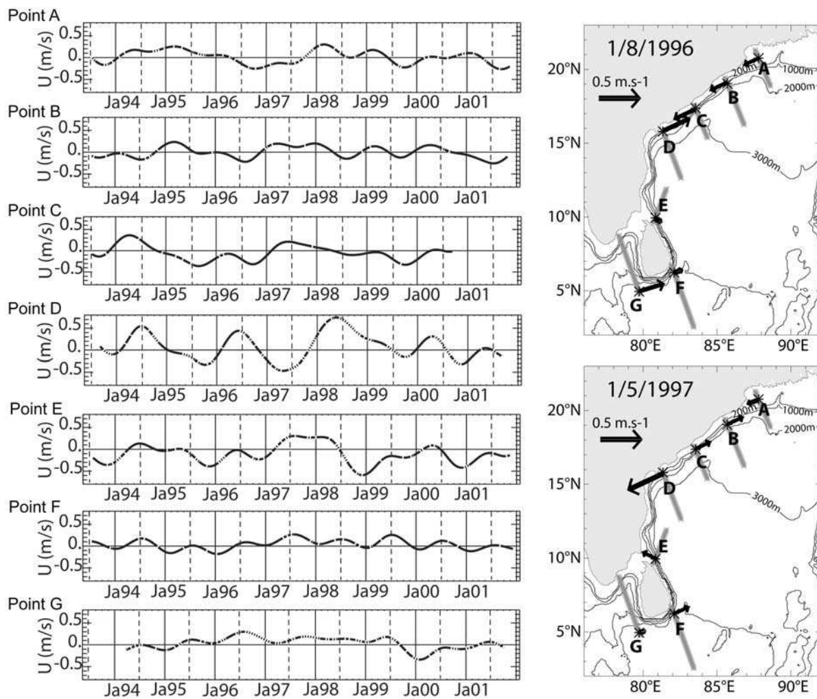
Figure 8. (left) Evolution during 1993–2001 of the interannual component of the altimetric cross-track geostrophic current anomaly for EICC points A–G. All currents are positive poleward (points A–F) and eastward (point G). The dotted portions show the gappy parts of the original (raw) time series. (right) Snapshots of the interannual EICC on 1 August 1996 and on 1 May 1997. The scale of the current vectors is indicated on the charts.
