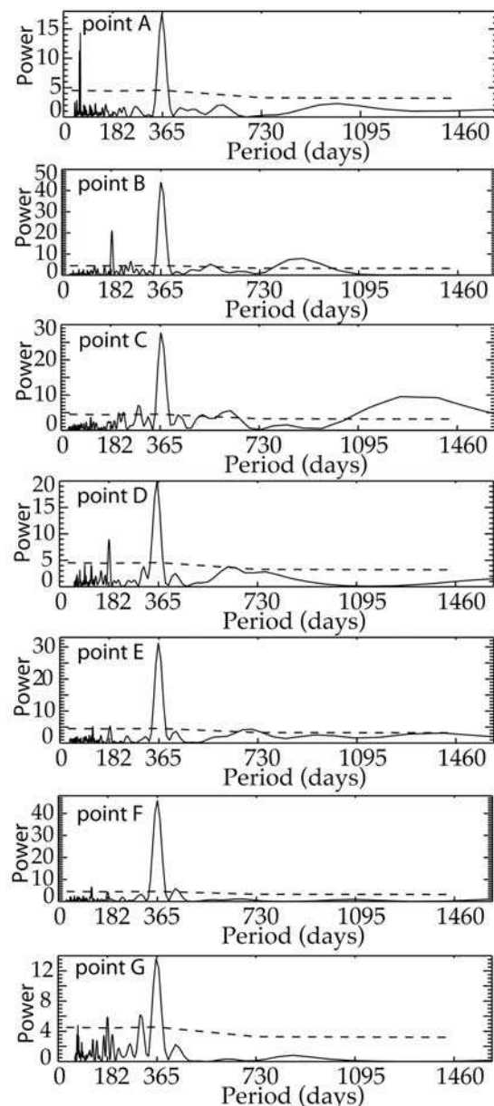
Figure 5. Lomb periodograms of the cross-track geostrophic surface current anomaly for each EICC point. The 95% significance level is indicated by dashed lines.
