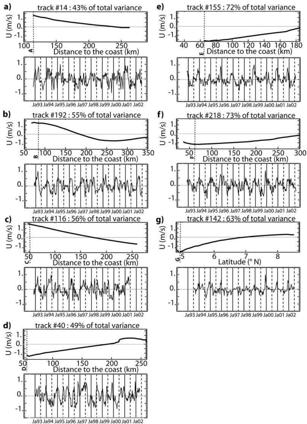
Figure 12. Spatial and temporal components of the first EOF mode of the cross-track geostrophic current anomaly for each altimetric track. The spatial component is plotted (a, b, c, d, e, f) as a function of the position along the altimetric track and (g) as a function of latitude. Superimposed in dotted line are the positions of the reference points A–G along the tracks. All currents are positive poleward (Figures 12a, 12b, 12c, 12d, 12e, and 12f) and eastward (Figure 12g). The percentage of variance explained by this mode is indicated at the top of Figures 12a, 12b, 12c, 12d, 12e, 12f, and 12g.
