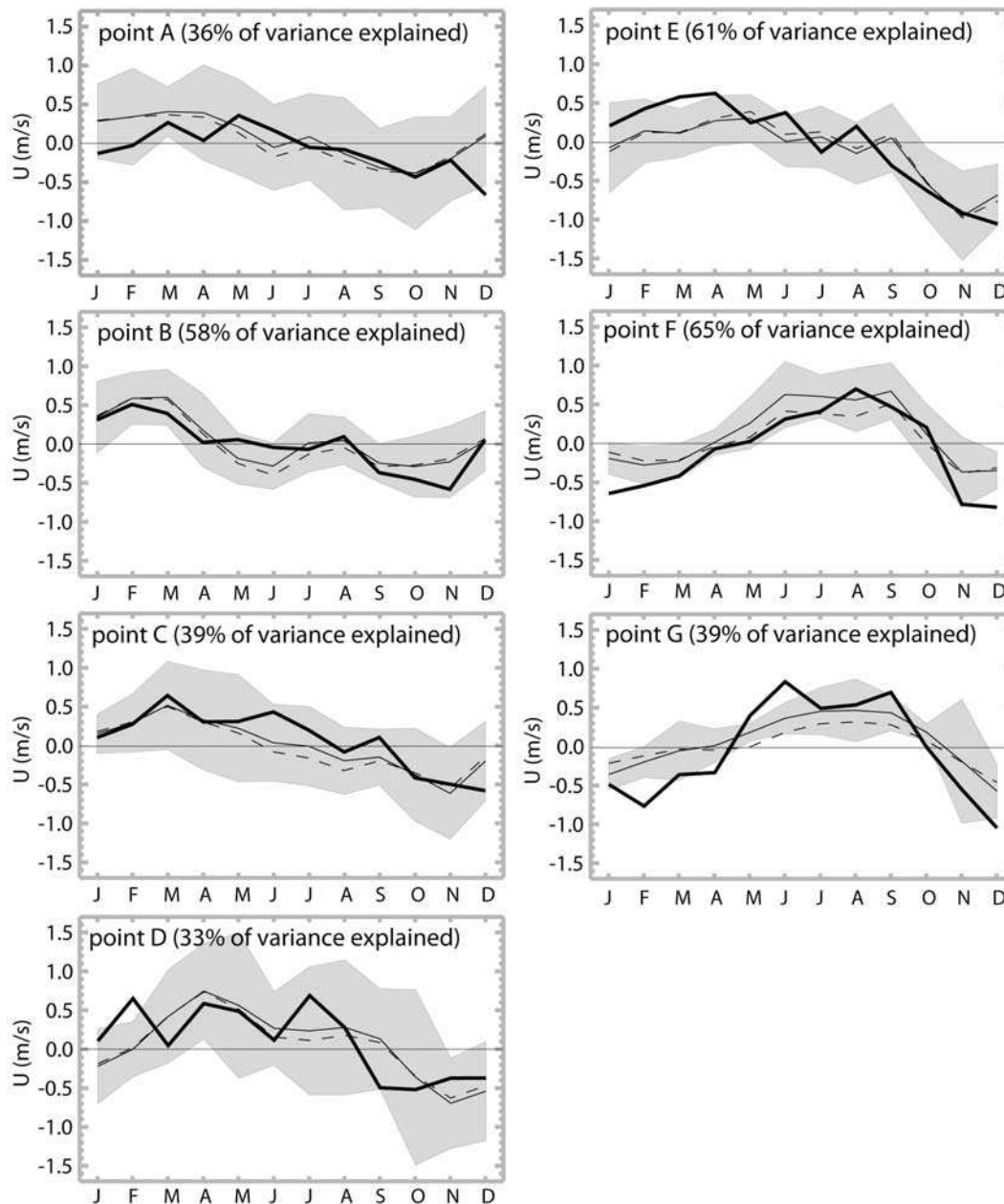
Figure 6. Seasonal climatology of surface current at the EICC points A to G (see map in Figure 1). The thick lines represent the Mariano et al. [1995] ship drifts projected in the alongshore direction, the thin dashed lines represent the altimetric cross-track geostrophic current anomaly we retrieved, and the thin solid lines represent the sum of altimetric cross-track geostrophic current anomaly and Ekman drift (estimated from ERS, the European Remote Sensing Satellite [ Bentamy et al. , 1996] scatterometer and projected in the cross-track direction). The gray shading is the interannual envelope of the total (geostrophic plus Ekman) current. All currents are positive poleward (points A–F) and eastward (point G). For each point, we indicate the percentage of the total variance of the geostrophic current explained by the seasonal climatology.
