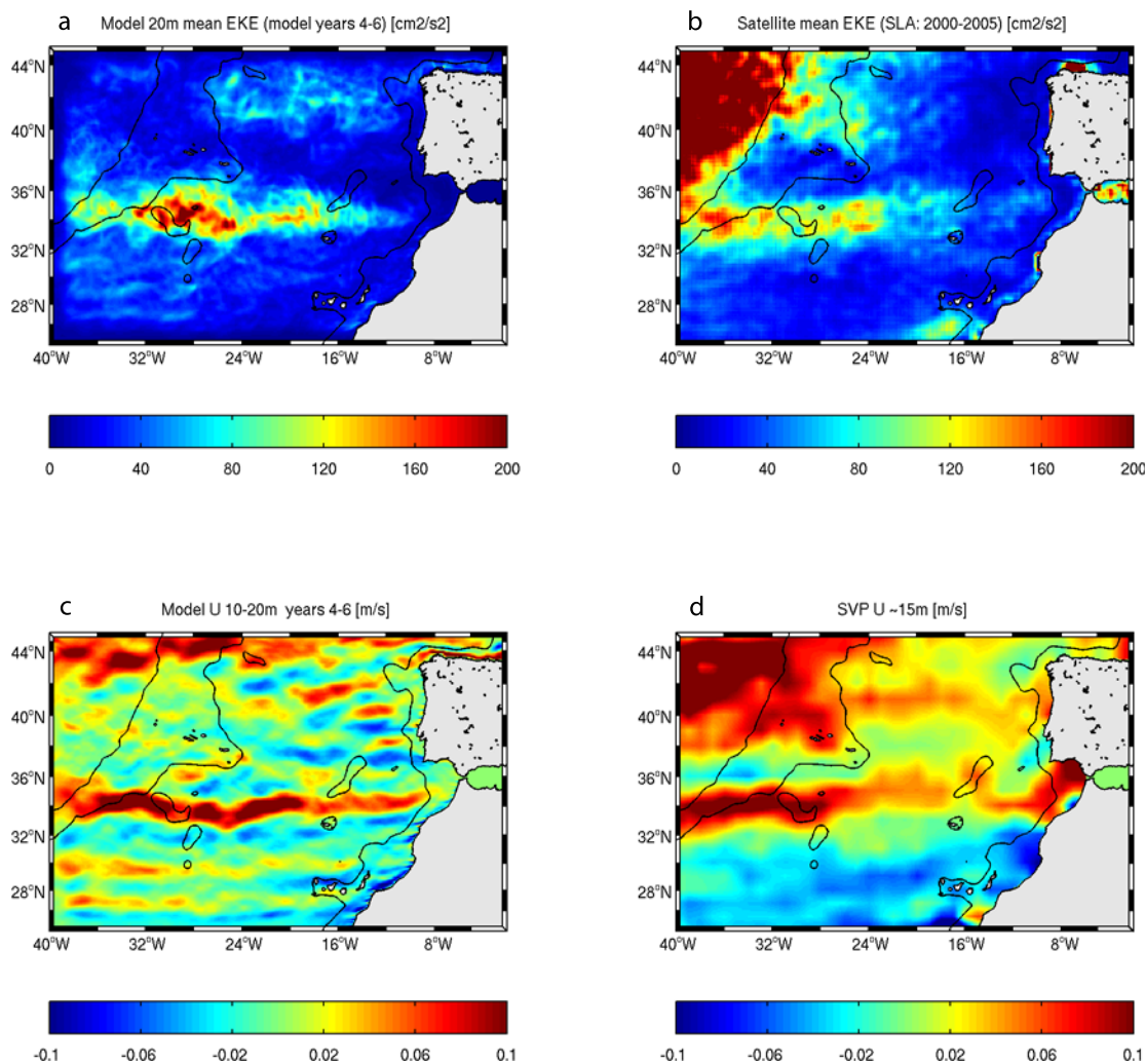
Figure 7. (a) LD 20-m EKE average for the period 4–6 model years. (b) EKE from merged satellite altimetry surface level anomalies (AVISO program) for years 2000–2005. (c) Mean U velocities (model years 4–6) for surface layer 10–20 m. (d) Climatology from the Surface Velocity Programme (surface drifting buoys drogued at 15 m).
